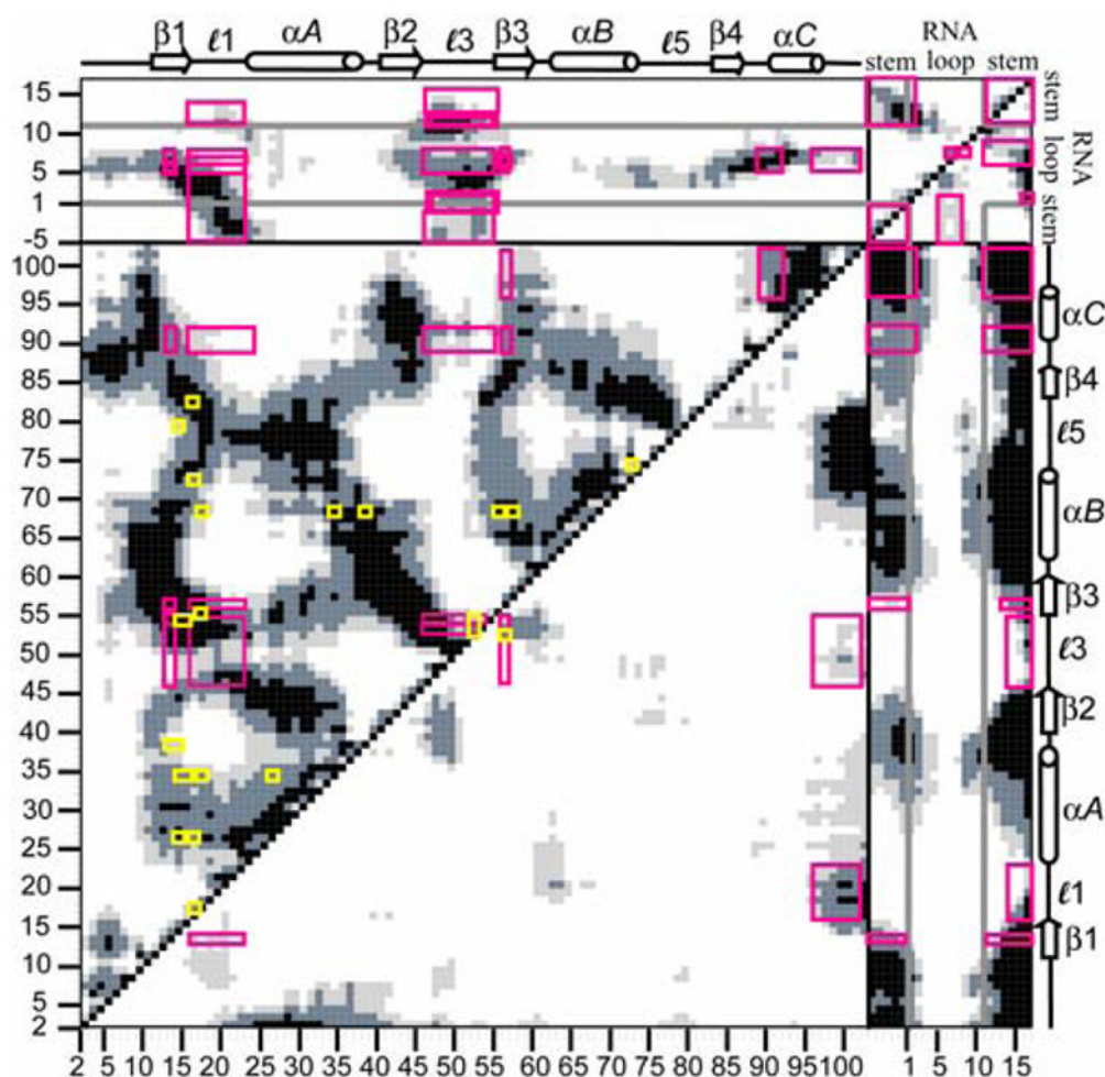
Figure 1. MD calculated collective atomic fluctuations for the U1A-RNA complex reduced to a residue by residue basis. Magnitudes of calculated correlations are indicated via a grey scale with black, slate gray and light gray regions corresponding to strong ( C_{ij} = \pm 0.75-1.00 ), moderate ( C_{ij} = \pm 0.50-0.75 ), and weak ( C_{ij} = \pm 0.25-0.50 ) cross-correlations, respectively. Upper triangle: positive correlations. Lower triangle: negative correlations. Magenta boxes indicate regions of the grid corresponding to residues and nucleotides implicated by biophysical studies as being involved in cooperative networks. 8-15 Yellow boxes indicate positions of residues revealed to exhibit high covariance from the Crowder et al. 16 study of 330 RRM.
