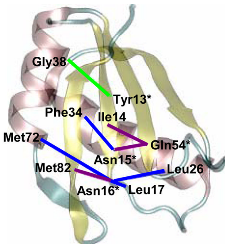
Figure 2. Cooperative interactions related to the U1A-RNA binding interface predicted from both MD calculated fluctuations and statistical covariance analysis for U1A. Residues directly in contact with RNA are indicated by an asterisk *. The magnitude of fluctuational covariance between residues corresponds to the line coloring: Purple: C_{ij} = \pm 0.75-1.00 ; Blue: C_{ij} = \pm 0.50-0.75 ; Green: C_{ij} = \pm 0.25-0.50 .
