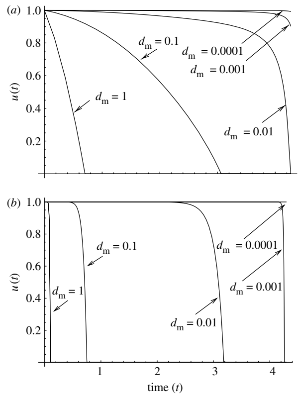
Figure 10. The optimal controls \bar{u}(t) for \alpha < 1 and various values of d_m . (a) \alpha=0.1 , the optimal times to target are 4.37, 4.35, 4.28, 4.27 and 4.27 for d=1; 0.1; 0.01; 0.001 and 0.0001 , respectively. (b) \alpha=0.9 , the optimal times to target are 4.36, 4.31, 4.28, 4.27 and 4.27. The other parameters are a=2 , u=0.1 , \sigma=10 and u_m=0.01 .
