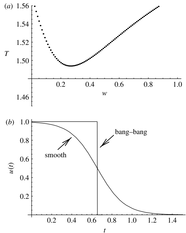
Figure 4. Does bang-bang work in the \alpha < 1 case? (a) The time to target, T , as a function of parameter w in formula (4.2). The other parameters are a=2 , \sigma=10 , \alpha=0.5 , u_m=1 , \mu=10^{-1} . (b) The control function, u_1(t) , corresponding to the best value of w . Also, the best bang-bang control for these parameters is shown. The time to target for the bang-bang control is T \approx 1.57 . For the function u_1(t) , it is T \approx 1.49 .
