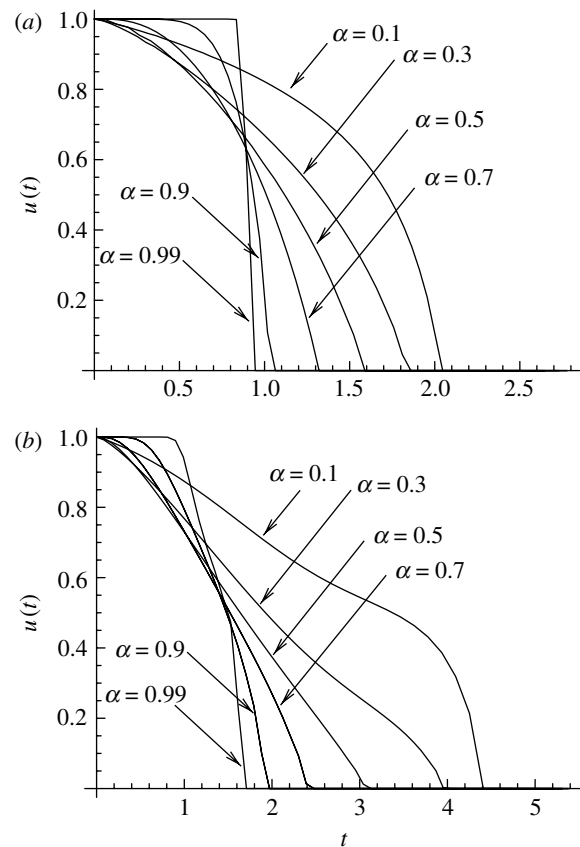
Figure 8. The optimal control found by the SQP method, for different values of \alpha < 1 , for (a) a one-step process and (b) a two-step process. The other parameters are a=2, \sigma=10, u_m=1, \mu=10^{-1} .
