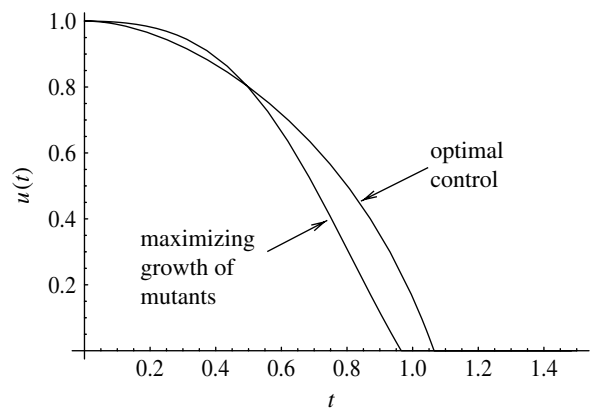
Figure 7. The optimal control found by the iterative method, compared to the function u(t) found from formula (4.3), which maximizes the growth of x_2(t) . The parameters are a=2, \alpha=0.5, \sigma=2, u_m=1, \mu=10^{-1} .
