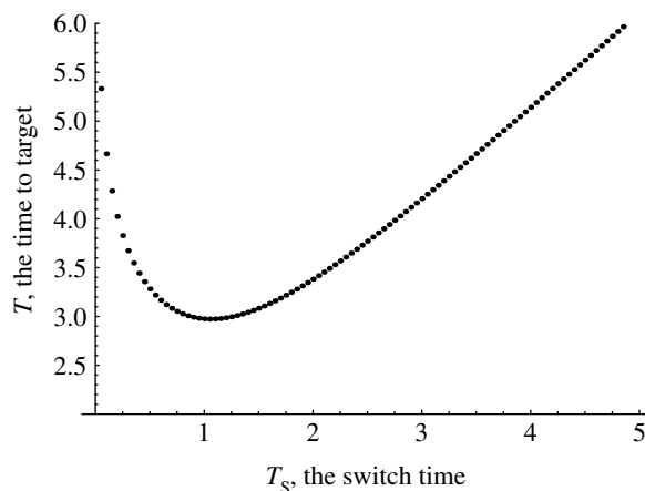
Figure 2. The minimum time to target, T , for different values of the switch time, T_s . The parameters are a = 2 , \sigma = 10 , \alpha = 2 , u_m = 1 , \mu = 10^{-7} .
