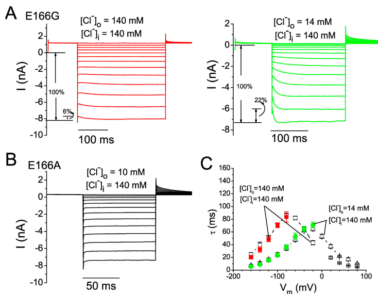
Figure 6. Extracellular CPA effects on the E166G and E166A mutants. (A) Recordings of the E166G mutant in two ionic conditions as indicated, with 10 mM CPA in the pipette. Voltage protocol is the same as that shown in the inset of Fig. 2. The percentage of the hyperpolarization-induced current out of the whole steady-state inward current ranged from 5.1–7.5% in the symmetrical 140-mM \text{Cl}^- condition and from 20.5–23.2% in the 140-/14-mM \text{Cl}^- condition. (B) Recordings of E166A with 10 mM CPA in the pipette. No hyperpolarization-activated current is noted at very negative voltages, even in low [\text{Cl}^-]_o (10 mM). (C) Time constants of the current-activating process shown in A (color symbols) upon stepping the potential from +80 mV to the various test voltages. Only the last several hyperpolarization voltages were able to generate a prominent current activation for a single-exponential fit. For comparison, the time constants presented in Fig. 5 B are reproduced (open symbols).
