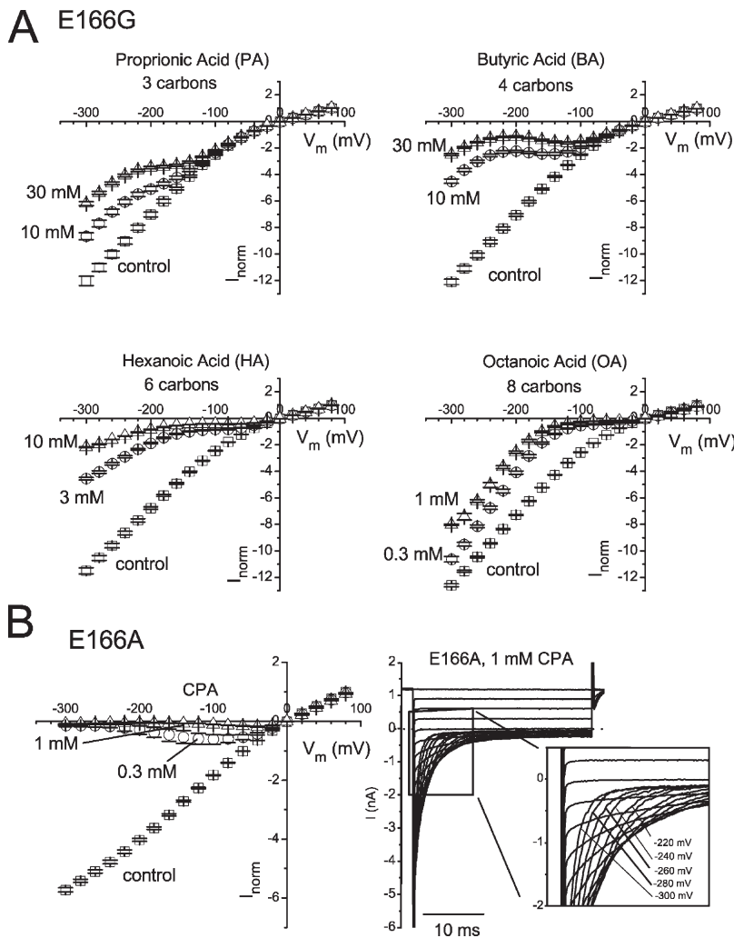
Figure 7. Steady-state I-V curves ( -300 to +80 mV) of E166G and E166A in symmetrical 140 mM \text{Cl}^- . (A) I-V curve of E166G constructed in the absence (control) and presence of two concentrations of the indicated fatty acids. The measured current was normalized to that obtained in the control condition at +80 mV. Notice that various fatty acids with different molecular lengths all punch through the pore of the E166G mutant. (B) I-V curves of E166A in the absence and presence of CPA. An example of the E166A recording in the presence of 1 mM CPA is shown on the right.
