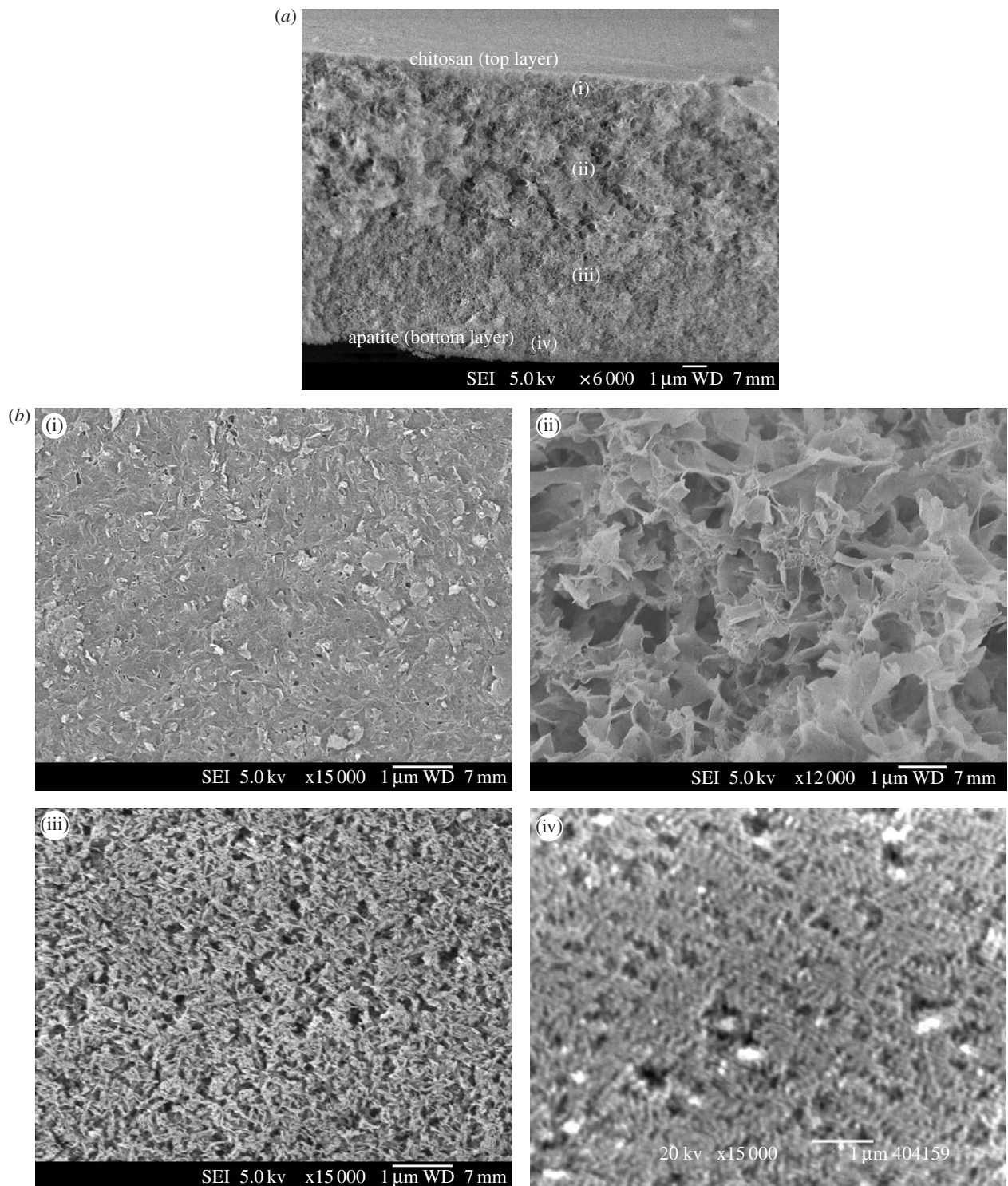
Figure 7. (a) Cross-section of HS70 hybrid nanostructured film showing (b) several levels of architecture—(i) mainly chitosan on the top of the film and (ii) the subsurface, (iii) chitosan–HA interwoven structure and (iv) assembled nHA at the bottom. Scale bar, 1 μm.
