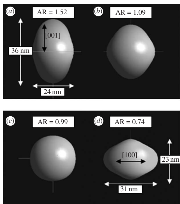
Figure 3. Crystallographically refined crystallite shapes for (a) HS00 (control, 0 \text{ mg l}^{-1} ), (b) HS20 ( 20 \text{ mg l}^{-1} ), (c) HS40 ( 40 \text{ mg l}^{-1} ) and (d) HS70 HA-chitosan hybrid nanoparticles ( 70 \text{ mg l}^{-1} ).
