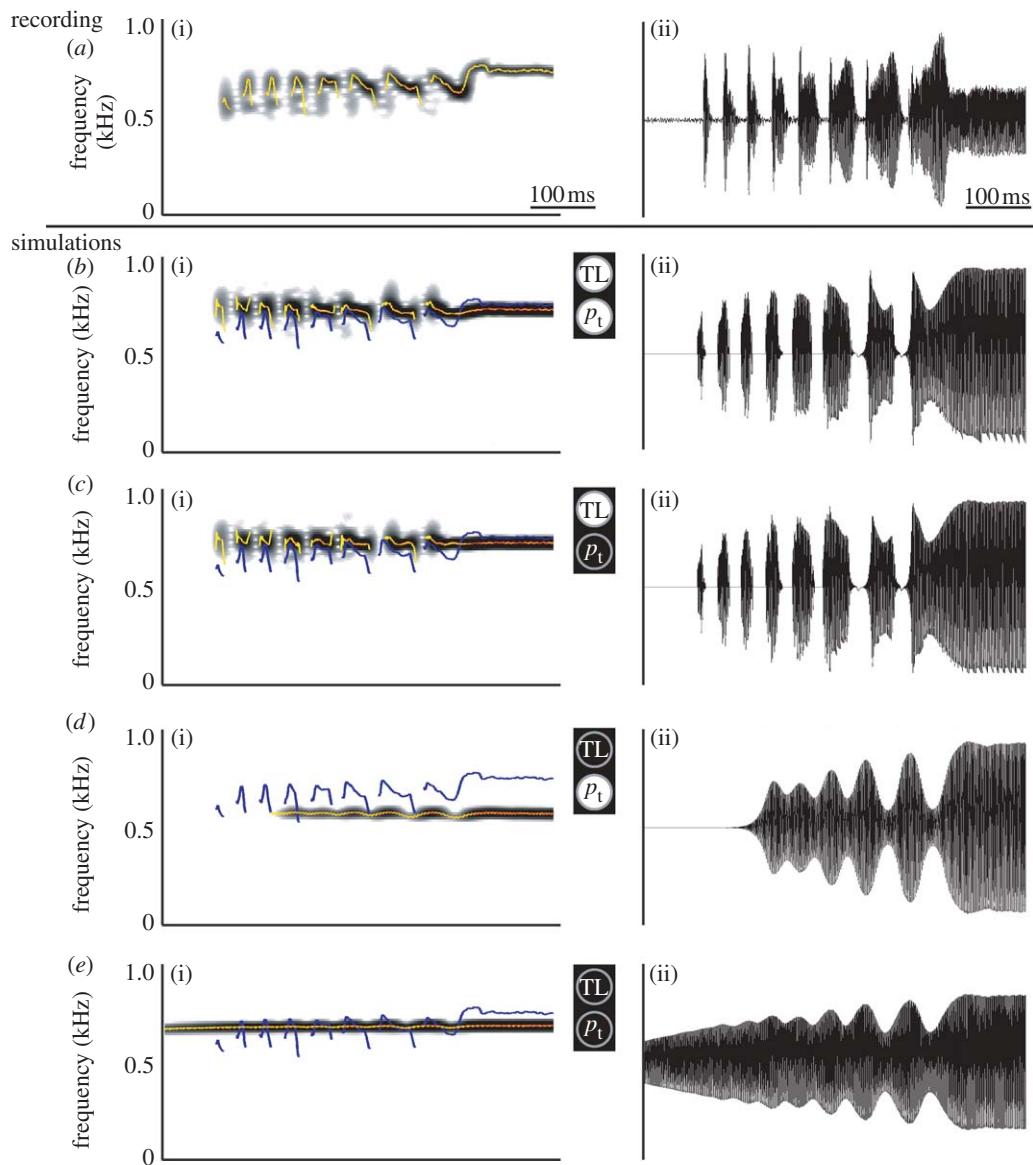
Figure 6. The effect of control parameters on the trill. (a) Recorded sound in vivo . (b–e) Model simulations with (c) no transmurial pressure, (d) no TL activity and (e) no transmurial pressure and no TL activity. In (c), the rest areas are constant ( 0.3 \text{ mm}^2 ). In (d), Q(t)=1 (see equation (4.9)) and rest areas are constant ( 0.3 \text{ mm}^2 ). Superimposed on spectrograms are: blue line, f_0 analysis of recorded coo in (a); yellow–red line, f_0 analysis of current signal. (a(i)–e(i)) sound spectrograms, (a(ii)–e(ii)) sound oscillograms.
