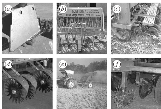
Figure 2. Various equipments for planting wheat no-till in RWC. (a) inverted T coulter, (b) Indian no-till drill using inverted T, (c) disc-type planter, (d) star-wheel punch planter, (e) 'happy planter' where straw picked up and blown behind seeder and (f) disc planter with trash mover.
