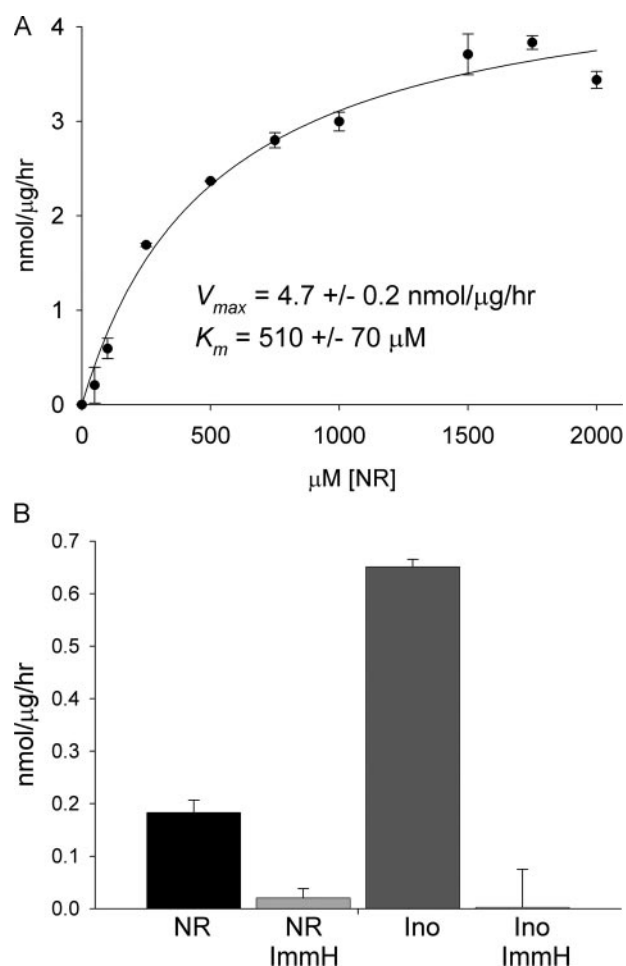
FIGURE 3. Mammalian NR phosphorylase activity is Pnp. A , crude mouse liver NR phosphorylase activity. B , specific activity of CACO-2 cell lysate phosphorylation of inosine ( Ino ) and NR without and with immucillin-H ( ImmH ) inhibition.
