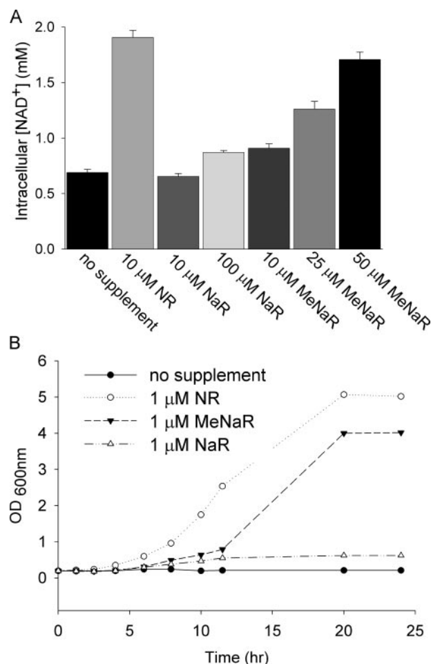
FIGURE 5. NaR utilization is facilitated by methyl ester modification. A, intracellular NAD + concentrations of wild-type yeast supplemented with NR, NaR, or meNaR at the indicated concentrations. B, de novo mutant bnal was grown for 18 h in SDC and then grown to exhaustion for 18 h in NA-free SDC. It was then diluted to a starting A_{(600 \text{ nm})} of 0.2 in the specified media. Although 1 \mu\text{M} NR was the best at promoting bnal growth, meNaR supported bnal growth after a lag period and 1 \mu\text{M} NaR did not.
