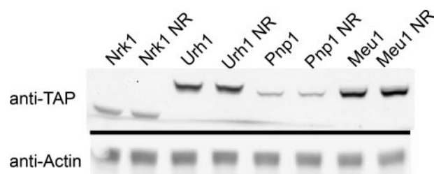
FIGURE 4. Relative protein abundance of NR salvage enzymes. Yeast strains, containing tandem affinity purification-tagged NR salvage enzymes, were grown in synthetic media without or with the addition of 100 μM NR. The relative abundance of the proteins, Meu1 > Urh1 > Nrk1 > Pnp1, was determined by Western blotting with an anti-tandem affinity purification antibody CAB1001 (Open Biosystems). Half of the blot was probed with anti-actin antibody as a loading control.
