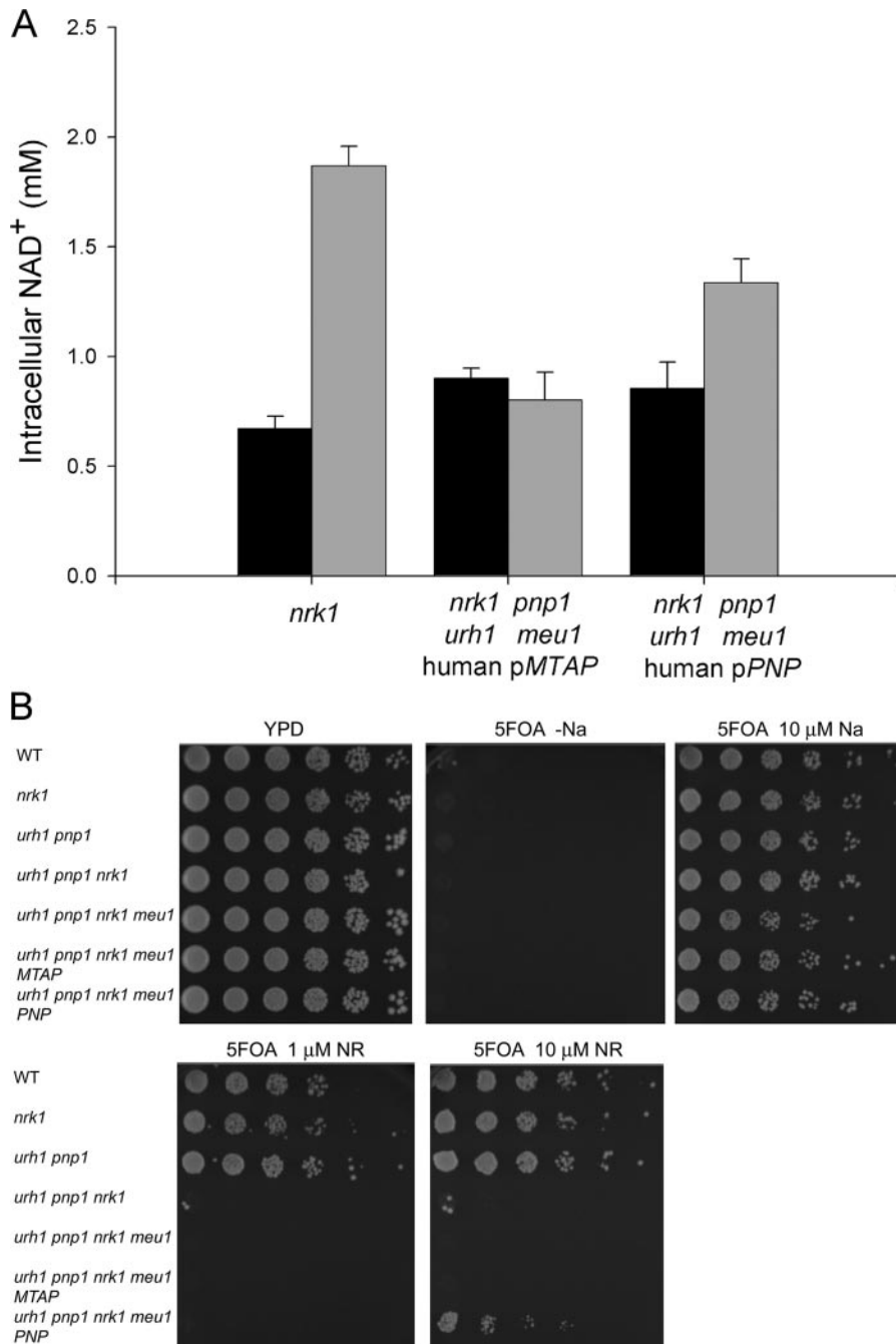
FIGURE 2. Human Pnp but not Mtap functions in yeast NR utilization. A , intracellular NAD + concentrations of the indicated genotypes were measured in NA-free SDC media (black bars) and in NA-free SDC media plus 100 μM NR (gray bars). pMTAP and pPNP indicate the addition of a pRS327 plasmid encoding a human cDNA fused to the yeast PNP1 promoter. Expression of human Pnp allows Nrk1 -independent NR utilization. B , all strains are gene silencing-deficient on medium without NA and are gene silencing-proficient on medium with 10 μM NA. 10 μM NR restores gene silencing to wild-type (WT) yeast but not yeast strains lacking both NR salvaging pathways. Human Pnp but not Mtap provides a partial rescue of the gene silencing deficiency, indicating function in NR salvage.
