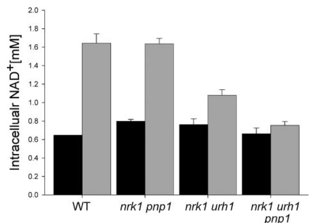
FIGURE 6. Urh1 is principally responsible for Nrk1-independent NaR/meNaR utilization. Intracellular NAD + concentration of yeast strains was supplemented with 50 \mu\text{M} meNaR. The urh1 deletion from nrk1 greatly reduces meNaR utilization, which is eliminated by deletion of nrk1 , urh1 , and pnp1 . WT, wild type.
