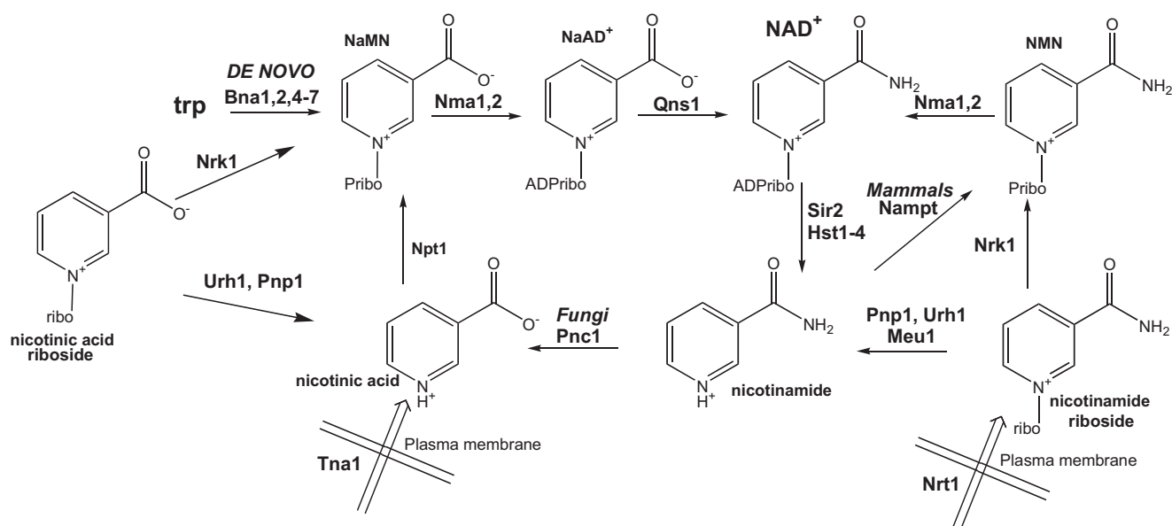
FIGURE 1. NAD + biosynthetic pathways in S. cerevisiae and mammals. NAD + is synthesized from tryptophan by the de novo biosynthetic pathway and from vitamin precursors, NA, Nam, and NR, through salvage pathways (1, 44). Salvage pathways in mammals and yeast differ in the utilization of Nam. Yeast convert Nam to NA via the nicotinamidase, Pnc1, whereas mammals convert Nam to nicotinamide mononucleotide (NMN) through the activity of the nicotinamide phosphoribosyltransferase, Namp1. In yeast, NR is salvaged via the Nrk1 pathway and the Urh1/Pnp1 pathway with slight flux through Meu1 (16). In yeast, NaR is salvaged by Nrk1 and the Urh1/Pnp1 pathway (20). According to the data in this study, mammalian Nrk-independent NR salvage relies solely on Pnp and, in yeast, Nrk-independent usage of NaR relies principally on Urh1. Urh1 is now classified as an NR hydrolase, with lower activity on uridine and NaR. ribo , riboside; ADPribo , ADP-ribose.
