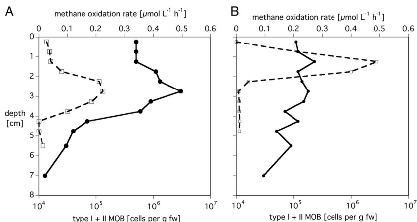
FIG. 4. Abundances of type I and II methanotrophs as determined by FISH (circles) together with the corresponding average methane oxidation rates (squares) for littoral (A) and profundal (B) sediments. fw, fresh weight.
