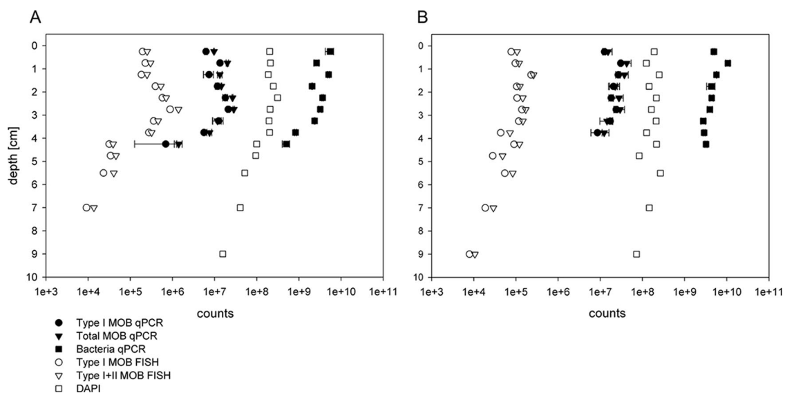
FIG. 3. Abundance of methanotrophs in littoral (A) and profundal (B) sediments. MOB as quantified by FISH (cells per g of sediment [wet weight]) and by qPCR (cells per g of sediment [wet weight]). Type I MOB (determined with M \gamma 84 and M \gamma 705 for FISH and the LC type I assay for qPCR), total numbers of MOB (determined with M \gamma 84, M \gamma 705, and M \alpha 450 for FISH and the MTOT assay for qPCR), and total bacterial numbers (determined by DAPI counts and 16S rRNA gene qPCR) are shown.
