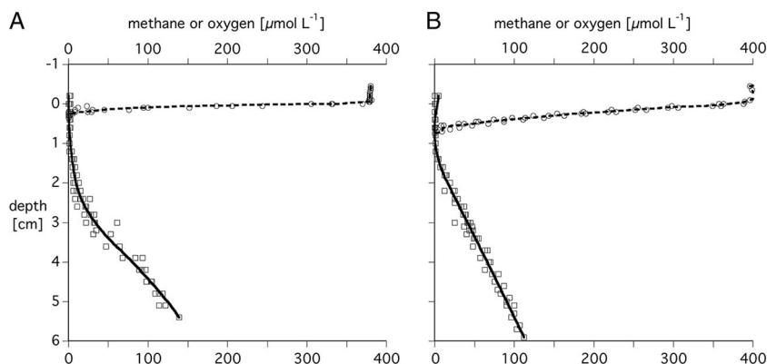
FIG. 1. Concentration profiles of oxygen (circles) and methane (squares) in littoral (A) and profundal (B) sediments. Lines indicate the means of three oxygen measurements and the calculated best-fitting profile of methane concentration.
