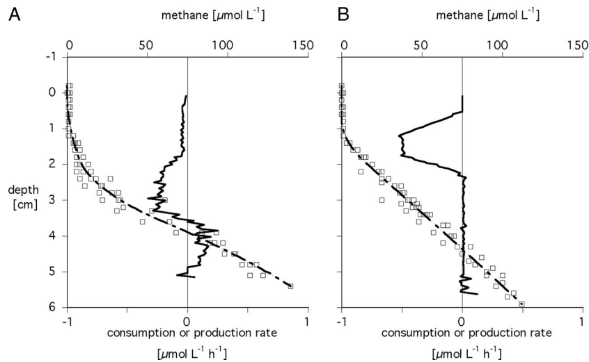
FIG. 2. Methane consumption and production rates (bold continuous line) calculated via Fick's second law of diffusion from the concentration profiles (dashed line) measured for littoral (A) and profundal (B) sediments. The individual data are plotted as squares.
