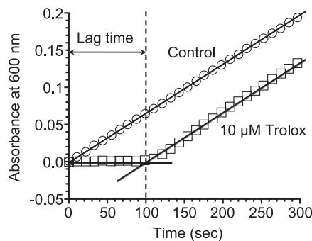
Fig. 1. Oxidation of ABTS (300 \mu M) by myoglobin (4.5 \mu M) with H 2 O 2 (250 \mu M) and its inhibition by Trolox (10 \mu M) at 25°C.
