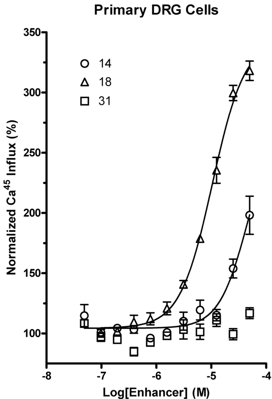
Figure 2. Dose-response kinetics of DHPs evaluated in primary DRG cells. Active DHPs retained similar kinetics in primary DRGs (e.g., 18 ), while inactive compounds were also inactive in DRGs (e.g., 31 ). Due to DMSO solvent sensitivity, the maximum DHP concentration evaluated in DRGs was 50 \mu M. The y-axis is normalized to the effect of capsaicin alone.
