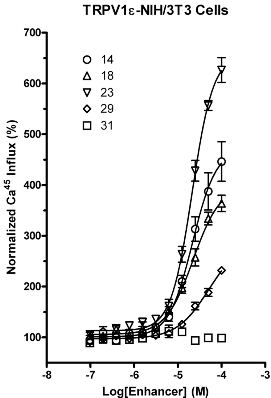
Figure 1. Representative dose-response kinetics of DHPs in the presence of a vanilloid evaluated in NIH3T3 cells ectopically expressing TRPV1. In the presence of 2 \mu M capsaicin, strong, dosedependent effects of some DHPs, e.g., compounds 14 , 18 , or 23 , were observed. Other DHPs were slightly active in the dose range evaluated (e.g., 29 ), while some were neutral even in the presence of capsaicin (e.g., 31 ). The y-axis is normalized to the effect of capsaicin alone.
