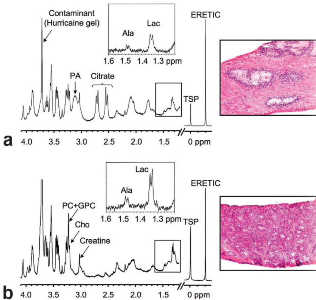
FIG. 1. Representative 1 H HR-MAS spectra and corresponding histopathologic sections of (a) benign predominantly glandular (40% glandular, 60% stroma) and (b) prostate cancer (70% Gleason 3+3) biopsy tissues. The major metabolites, TSP, and ERETIC resonances are shown. Lactate to alanine regions from 144-ms CPMG spectra are shown inset.
