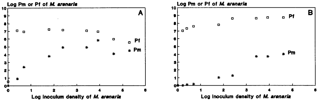
FIG. 1. Relationships between inoculum density of Meloidogyne arenaria eggs per 100 cm 3 soil and midseason (Pm) and final (Pf) densities of M. arenaria juveniles per 100 cm 3 soil in microplots. Each point is the mean of 10 replications, and both axes are log e scales. A) 1989. B) 1990.
