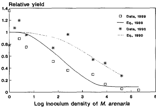
FIG. 3. Relationships between inoculum density of Meloidogyne arenaria per 100 cm 3 soil ( x ) and relative yield ( y ) in peanut pods (dry weight) in microplots. 1989: y = 0.088 + 0.91(0.90)^{(x-1)} for x > 1 and y = 1.00 for x \leq 1 ; maximum yield = 181.5 g; r^2 = 0.826 . 1990: y = 0.22 + 0.78(0.97)^{(x-1)} for x > 1 and y = 1.00 for x \leq 1 ; maximum yield = 193.0 g; r^2 = 0.794 . Each point (Data) is the mean of 10 replications, and lines (Eq.) indicate Seinhorst equations. The x-axis is log e scale.
