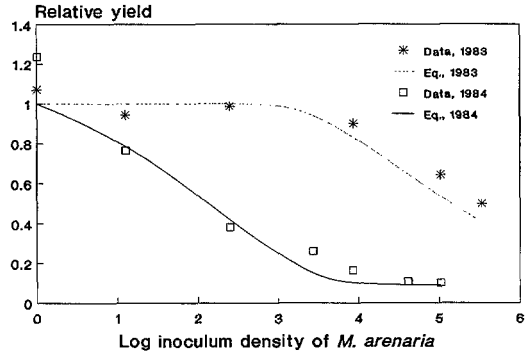
FIG. 4. Relationships between inoculum density of Meloidogyne arenaria per 100 cm 3 soil ( x ) and relative yield ( y ) in peanut pods (dry weight) in microplots. 1983: y = 0.33 + 0.67(0.99)^{(x-23)} for x > 23 and y = 1.00 for x \leq 23 ; maximum yield = 233.8 g; r^2 = 0.966 . 1984: y = 0.090 + 0.91(0.90)^x for x \geq 0 ; maximum yield = 493.6 g; r^2 = 0.912 . Each point (Data) is the mean of 10 replications, and lines (Eq.) indicate Seinhorst equations. The x-axis is log e scale.
