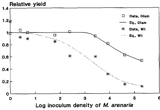
FIG. 2. Relationships between inoculum density of Meloidogyne arenaria per 100 cm 3 soil ( x ) and relative yield ( y ) in microplots, 1989. Plant diameter: y = 0.51 + 0.49(0.98)^{(x-23)} for x > 23 and y = 1.00 for x \leq 23 ; maximum yield 30.4 cm; r^2 = 0.985 . Foliage dry weight: y = 0.12 + 0.88(0.97)^{(x-1)} for x > 1 and y = 1.00 for x \leq 1 ; maximum yield = 237.6 g; r^2 = 0.913 . Each point (Data) is the mean of 10 replications, and lines (Eq.) indicate Seinhorst equations. The x-axis is log e scale.
