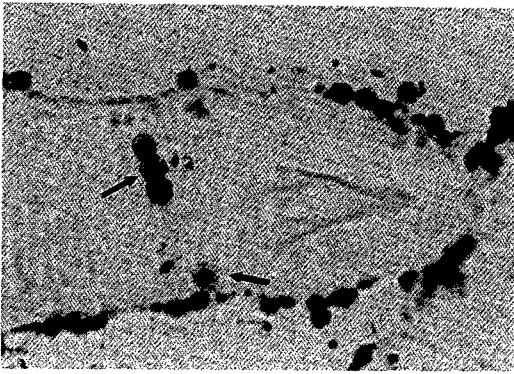
FIG. 6. Photomicrograph of the tail region of a squashed male of Meloidogyne arenaria parasitized by Pasteuria penetrans . Arrows mark mature, Gram-stained sporangia ( \times 920 ).
