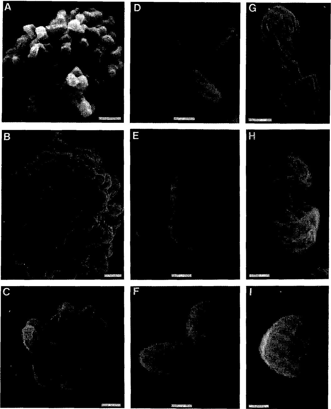
FIG. 2. Scanning electron micrographs of the developmental stages of Pasteuria penetrans . Scale bars = 1 \mu\text{m} . A) Early vegetative stage of a mycelial colony. B) Later stage of a mycelial colony, irregularly shaped and enlarged. C) Mycelial branches after breaking apart from the thallus cluster. D) Enlargement of mycelial branches and fragmentation into quartets. E) Early sporangial development, doublets beginning to form. F) Sporangium size increases and doublets become predominant. G) Endospore development within the sporangium continues. H) Nearly mature sporangia beginning to separate. I) Single mature sporangium with endospore inside.
