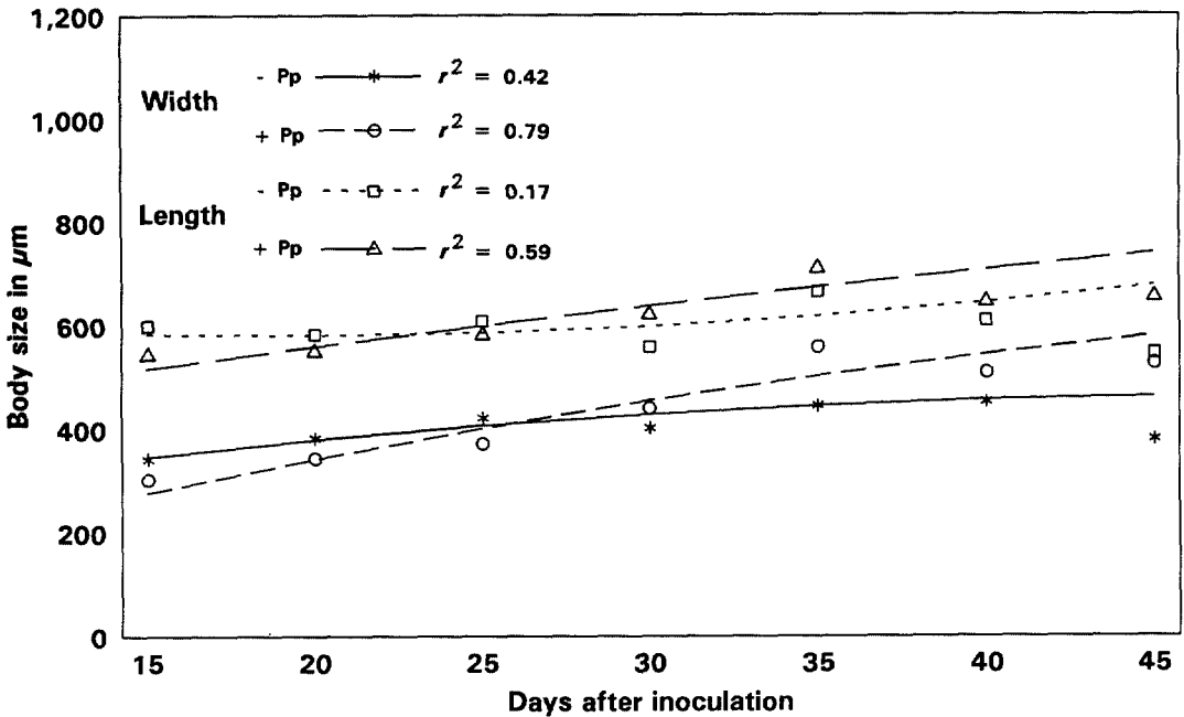
FIG. 5. Regression models (lines) and observed data points (from at least 10 observations) for width and length of Meloidogyne arenaria females uninfected or infected with Pasteuria penetrans at 30 C. Width, untreated: y = 215.89 + 10.43x - 0.11x^2 , r^2 = 0.42 . Width, treated: y = 45.56 + 17.28x - 0.12x^2 , r^2 = 0.79 . Length, untreated: y = 631.5 - 5.28x + 0.14x^2 , r^2 = 0.17 . Length, treated: y = 380.37 + 9.8x - 0.04x^2 , r^2 = 0.59 .
