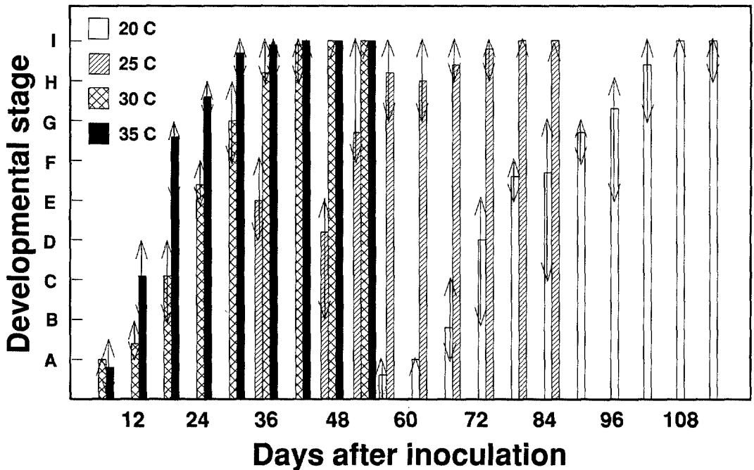
FIG. 3. Development of Pasteuria penetrans in females of Meloidogyne arenaria on Lycopersicon esculentum at 20, 25, 30, and 35 C over time. After inoculation refers to inoculation of tomato with second-stage juveniles of M. arenaria with endospores attached. The developmental stages are listed in the legend of Figure 2. Bars represent the means of more than 10 females observed at each sampling time. Vertical arrows show the range of developmental stages present at each sampling time.
