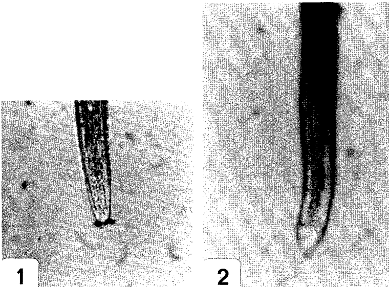
FIGS. 1,2. Anterior end of Meloidogyne javanica second-stage juveniles. 1) Labelling with gold-Concanavaline A. 2) Labelling with gold-conjugated fucosylated-BSA (bovine serum albumin).
