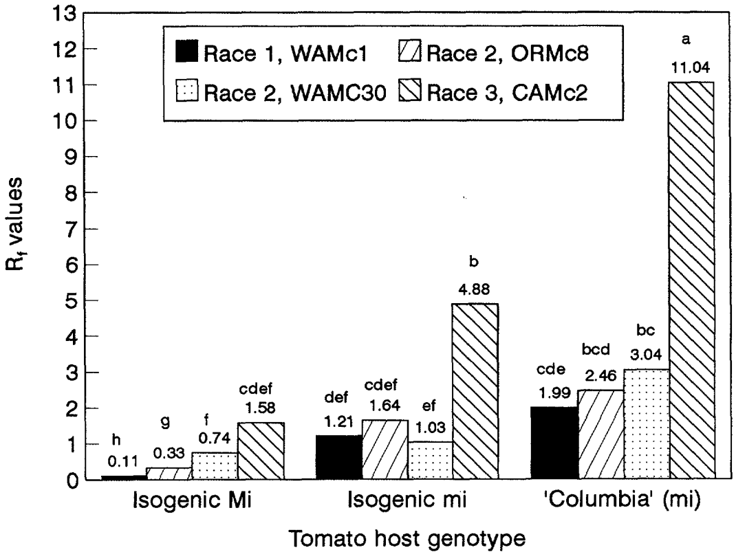
FIG. 1. R_f values of different races of M. chitwoodi on tomato lines Sun 6082 (isogenic Mi ), Castlerock II (isogenic mi ), and the cultivar Columbia, an mi genotype. R_f values are shown at the top of each bar; values not sharing the same letter are statistically different at P < 0.05 according to Duncan's multiple-range test. R_f values are geometric means of 3 to 5 replicates.
