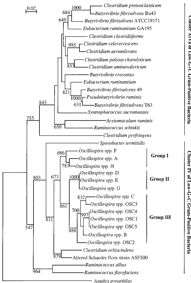
FIG. 2. Phylogenetic placement of partial 16S rDNA sequences, amplified with the Oscillospira -specific primer set OSCI, within the main rumen bacterial phyla. Previously cloned Oscillospira sequences are labeled OSC1 through OSC5. The sequences generated in this work are labeled A through H. The Aquifex pyrophilus sequence is used as the outgroup for rooting the tree. Numbers above each node are confidence levels generated from 1,000 bootstrap trees (5). The scale bar is in fixed nucleotide substitutions per sequence position.
