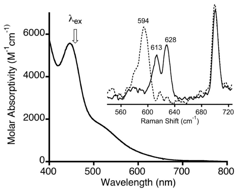
Figure 1. UV-vis spectrum ( -80\text{ }^\circ\text{C} ) and resonance Raman spectra (inset, -196\text{ }^\circ\text{C} , \lambda_{\text{ex}} = 457.9\text{ nm} as noted by arrow in the UV-vis spectrum; solid line = ^{16}\text{O} , dashed line = ^{18}\text{O} ) of [\text{LMe}_2\text{Cu}(\mu\text{-O})_2\text{Pt}(\text{PPh}_3)_2]\text{PF}_6 in 4:1 v/v THF/ \text{CH}_2\text{Cl}_2 . The peak at \sim 700\text{ cm}^{-1} is due to \text{CH}_2\text{Cl}_2 .
