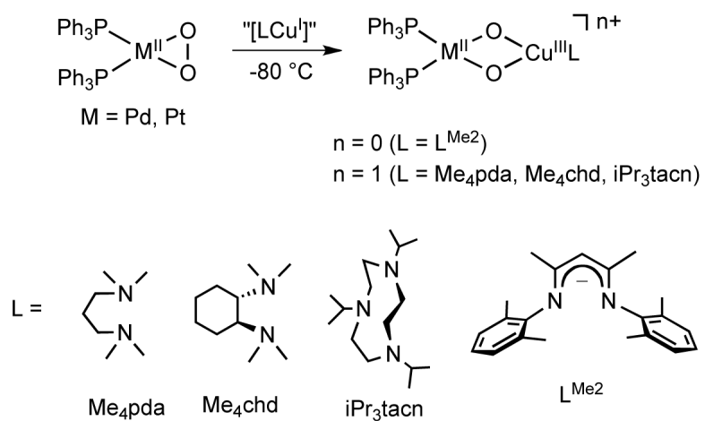
Scheme 1. Synthesis of heterobimetallic bis( \mu -oxo) complexes.
