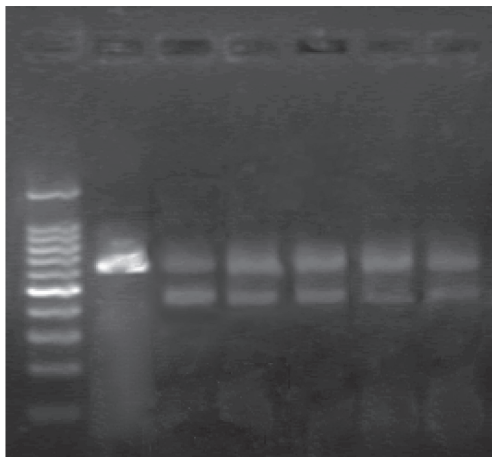
Figure 6 The MDRI mRNA level of K562/A02 cells with nanoparticles ( 5.0 \times 10^{-7} M Nano-Fe 3 O 4 or 2.0 \times 10^{-8} M Nano-Au) in the absence or presence of DNR (10 mg/L) Lane: 1, marker; 2, K562 (negative control); 3, K562/A02 (positive control); 4, Nano-Fe 3 O 4 ; 5, Nano-Au; 6, DNR with Nano-Fe 3 O 4 ; 7, DNR with Nano-Au.
