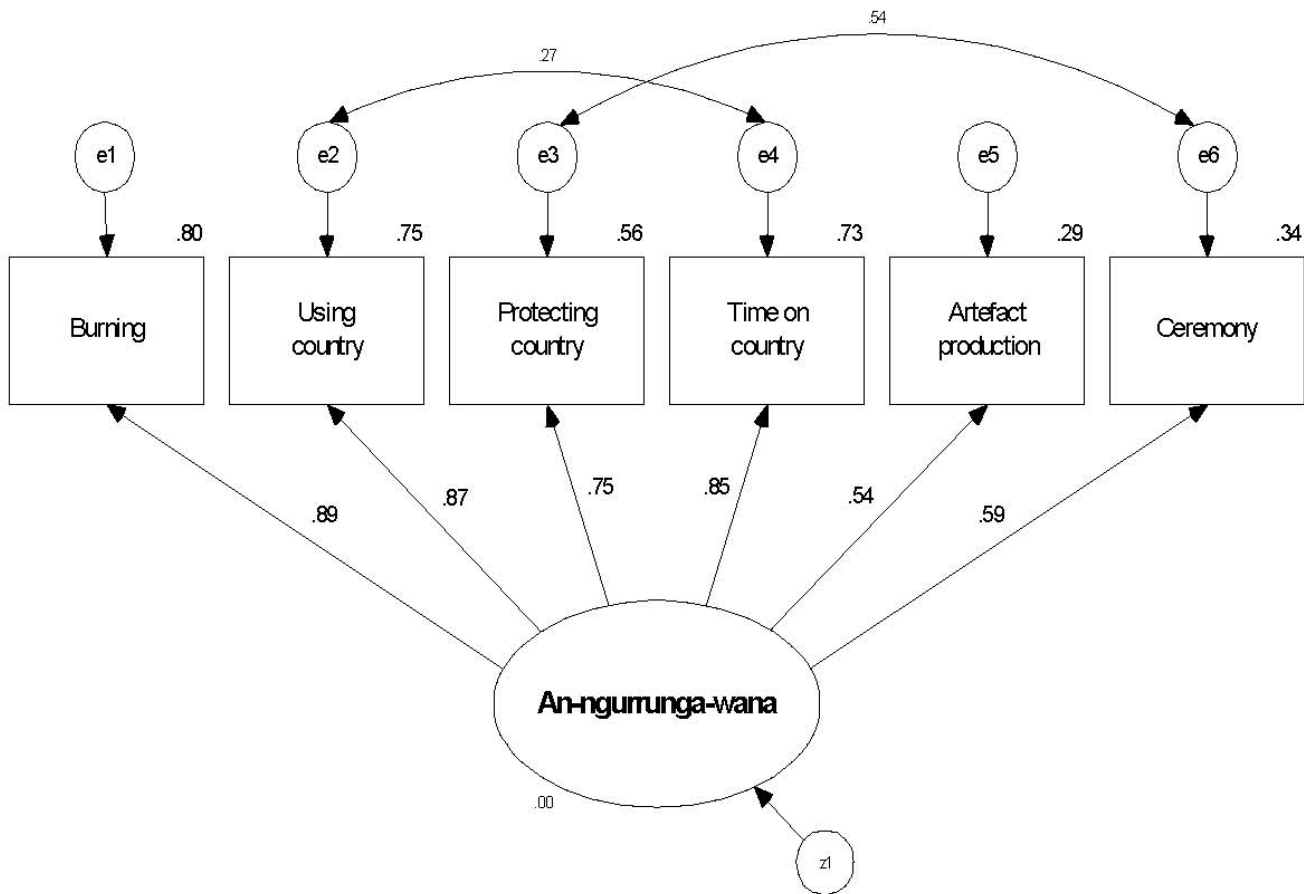
Figure 1 Fitted one factor congeneric model and standardised estimates of an-ngurrngna-wana .
