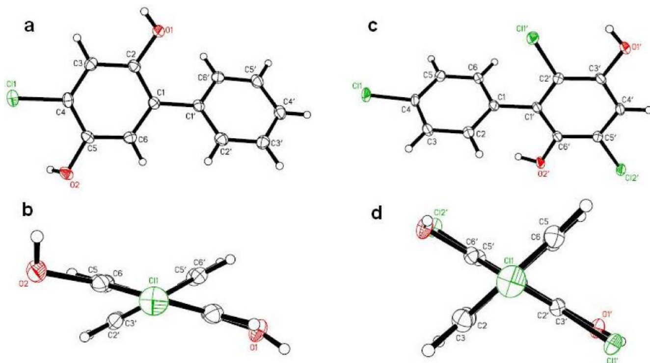
Figure 1. Molecular structures derived from the crystal structure of 13 and 20 (a) Molecular structure of 4-chloro-biphenyl-2,5-diol ( 13 ) showing the atom-labeling scheme and (b) view of 4-chloro-biphenyl-2,5-diol ( 13 ) along the C1–C1' axis illustrating the non-planar conformation of the molecule; (c) molecular structure of 3,6,4'-trichloro-biphenyl-2,5-diol ( 20 ) showing the atom-labeling scheme and (d) view of 3,6,4'-trichloro-biphenyl-2,5-diol ( 20 ) along the C1–C1' axis illustrating the non-planar conformation of the molecule. Displacement ellipsoids are drawn at the 50% probability level.
