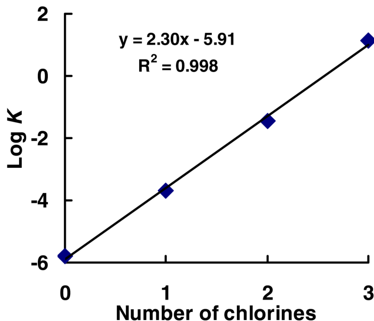
Figure 4. The equilibrium constant for the comproportionation reaction to form SQ^{\bullet-} increases with the number of chlorines on the oxygenated ring
