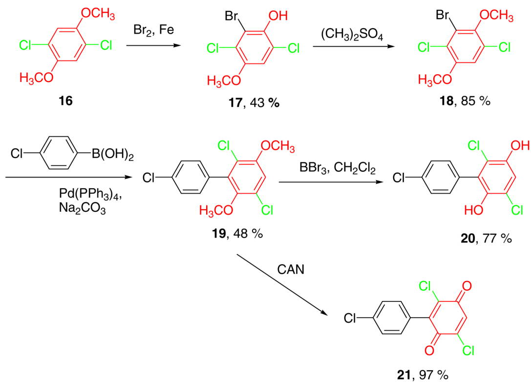
Scheme 2. Synthesis of PCB hydroquinones/quinones with two chlorines on the oxygenated ring
