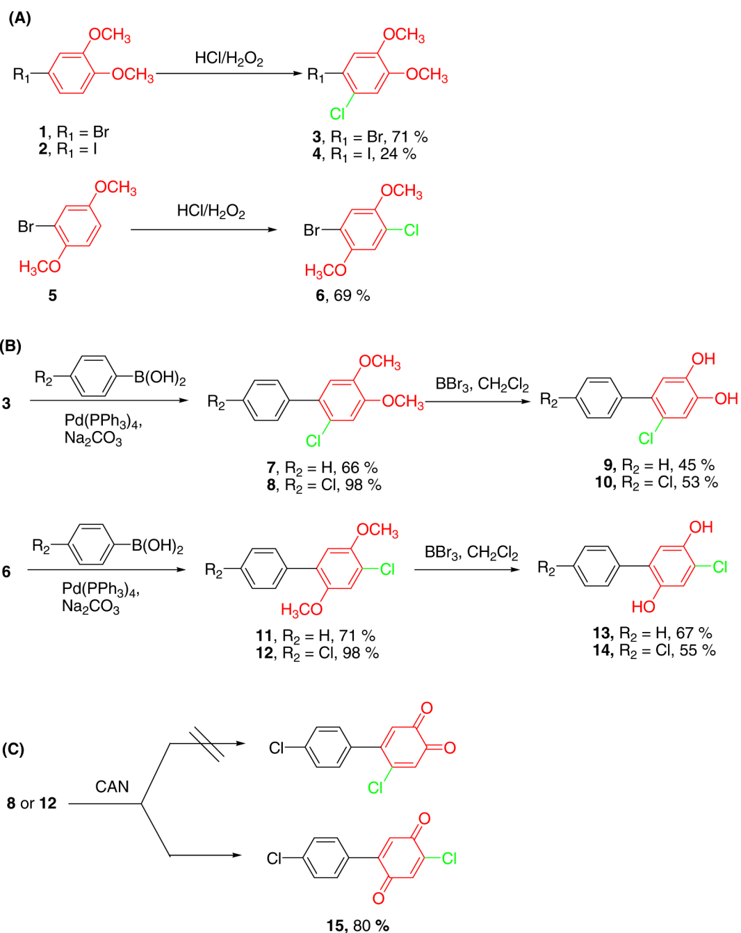
Scheme 1. Synthesis of PCB hydroquinones/quinones with one chlorine on the oxygenated ring
