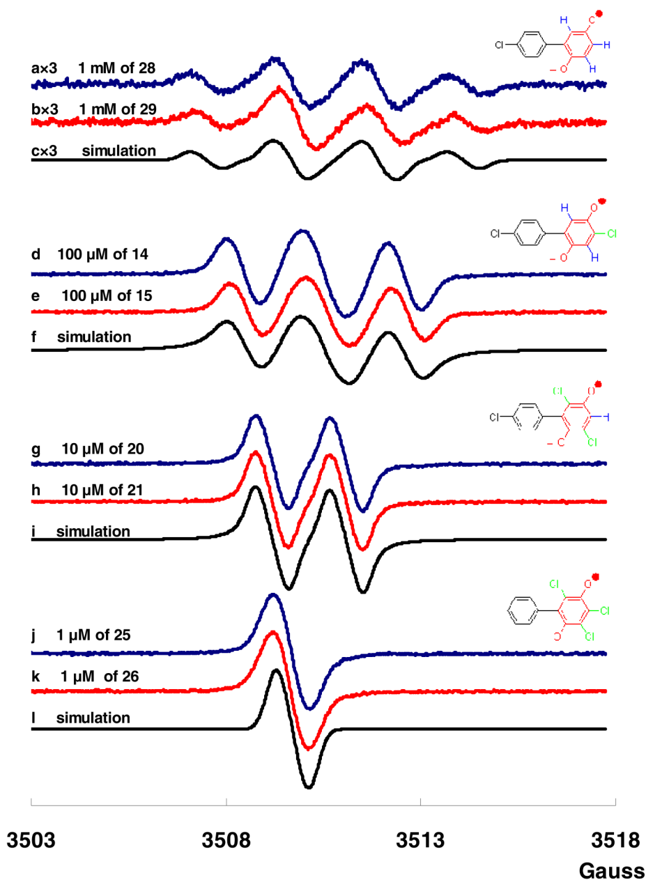
Figure 3. EPR spectra of semiquinones generated from PCB hydroquinones and quinones with differing numbers of chlorine on the oxygenated phenyl rings (a) SQ^{\bullet-} generated from 1 mM of 4'-chloro-biphenyl-2,5-diol ( 28 ) (yield: 0.000 092); (b) SQ^{\bullet-} generated from 1 mM of 2-(4-chloro-phenyl)-[1,4]benzoquinone ( 29 ) (yield: 0.000 12); (c) computer simulation of SQ^{\bullet-} with three hydrogens; (d) SQ^{\bullet-} generated from 100 \mu M of 4,4'-dichloro-biphenyl-2,5-diol ( 14 ) (yield: 0.004 5); (e) SQ^{\bullet-} generated from 100 \mu M of 2-chloro-5-(4-chloro-phenyl)-[1,4]benzoquinone ( 15 ) (yield: 0.003 5); (f) computer simulation of SQ^{\bullet-} with two hydrogens; (g) SQ^{\bullet-} generated from 10 \mu M of 3,6,4'-trichloro-biphenyl-2,5-diol ( 20 ) (yield: 0.026); (h) SQ^{\bullet-} generated from 10 \mu M of 2,5-dichloro-3-(4-chloro-phenyl)-[1,4]benzoquinone ( 21 ) (yield: 0.025); (i) computer simulation of SQ^{\bullet-} with one hydrogen; (j) SQ^{\bullet-} generated from 1 \mu M of 3,4,6-trichloro-biphenyl-2,5-diol ( 25 ) (yield: 0.23); (k) SQ^{\bullet-} generated from 1 \mu M of 2,3,5-trichloro-6-phenyl-[1,4]benzoquinone ( 26 ) (yield: 0.23);
