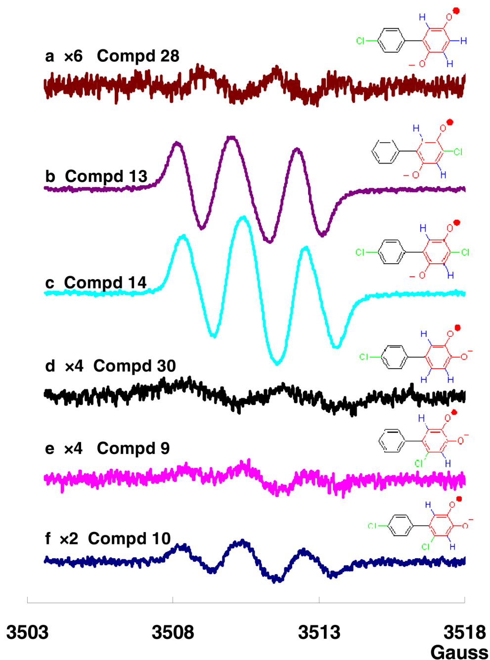
Figure 2. EPR spectra of semiquinones generated from PCB hydroquinones with differing numbers and positions of chlorine on the phenyl rings
