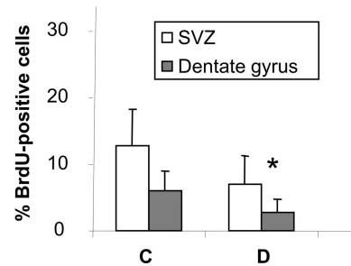
Fig. 1. ( Upper ) Thionin coloration of the CA1 hippocampus from control (C) and B-vitamin-deficient (D) rats at 21 days of age (40 \times magnification). ( Lower ) Percentage of BrdU-positive cells (after a single i.p. injection of 50 mg/kg) among total cells counterstained by DAPI in the subventricular zone (SVZ) and the hippocampal dentate gyrus. Data are reported as means \pm SD ( n = 7 ). C, control; D, deficient diet. *, P < 0.05 (statistically significant difference versus control, ANOVA, Fisher's test).
