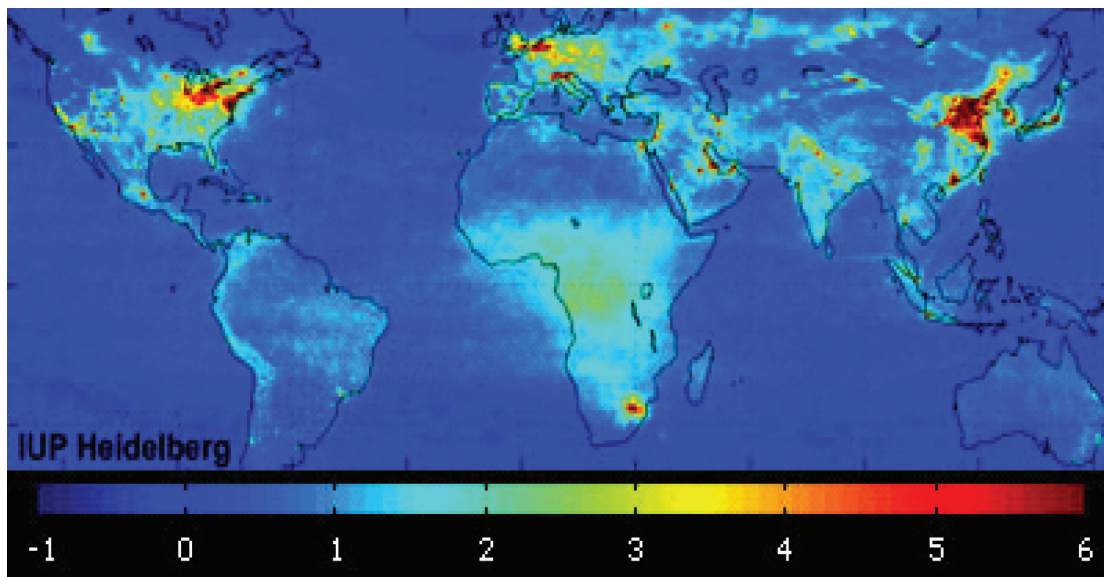
Figure 2 Global mean tropospheric nitrogen dioxide (NO 2 ) vertical column density between January 2003 and June 2004. Concentrations increase with color intensity: blue, lowest NO 2 concentrations; deep red, highest NO 2 concentrations. Eighteen-month average taken from www.esa.int/images/pollution_global_L .
