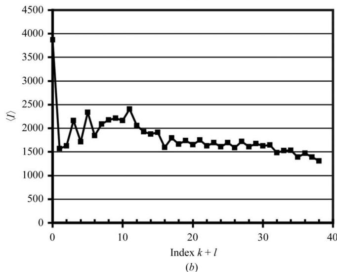
Figure 2 Layer-averaged intensity as a function of index k + l for (a) the observed uncorrected intensities and (b) the corrected intensities using the procedure described in the text.
