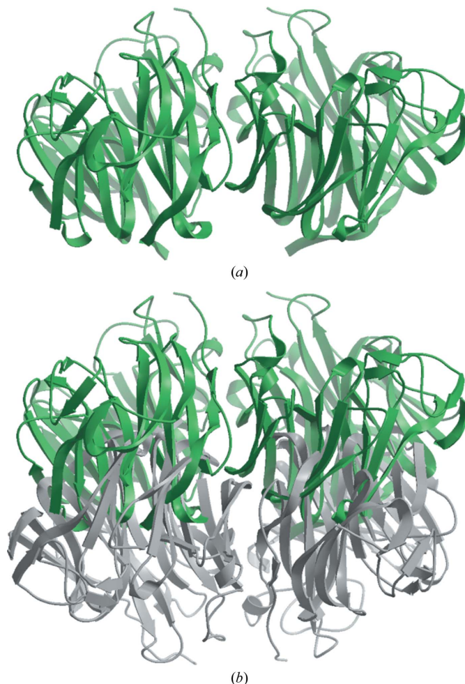
Figure 3 18NA molecules in ribbon representation in the crystal lattice domains: (a) in one lattice domain as a dimer (green), (b) in two lattice domains as high-occupancy and low-occupancy dimers (green and grey, respectively).
