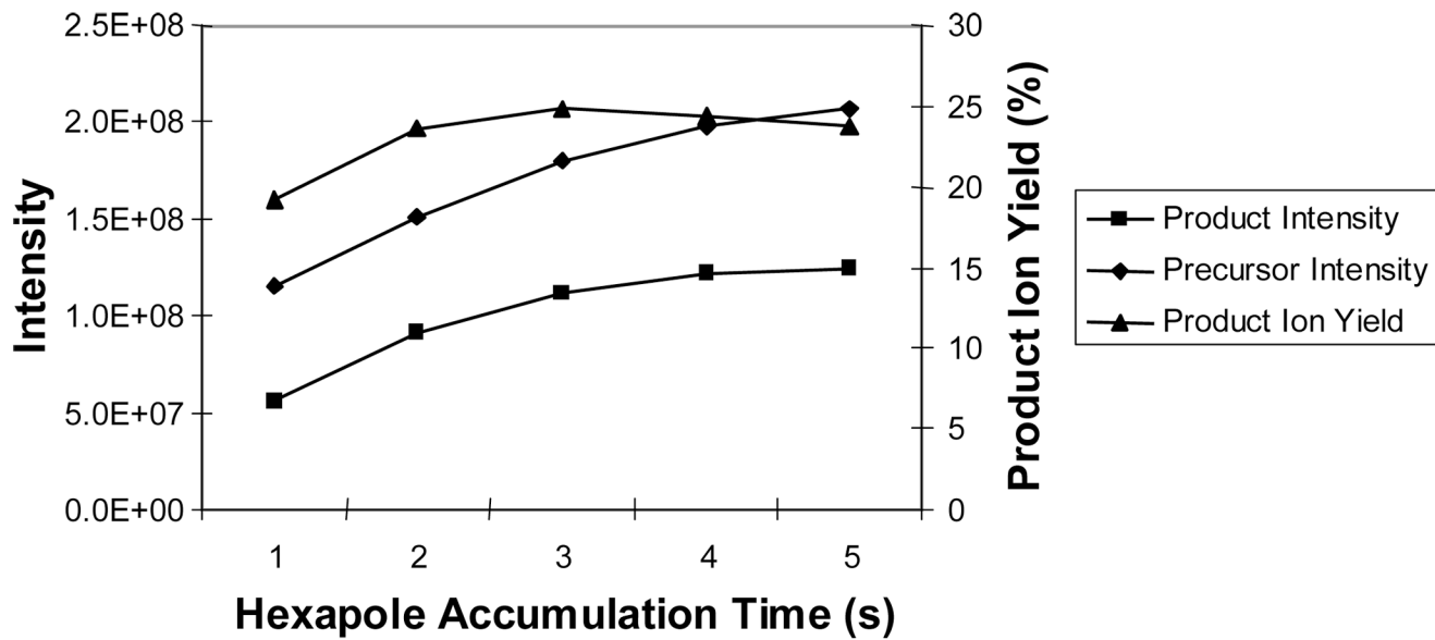
Figure 7. Efficiency of product formation (right axis) and precursor/product intensities (left axis) as a function of precursor accumulation time in the external hexapole.
