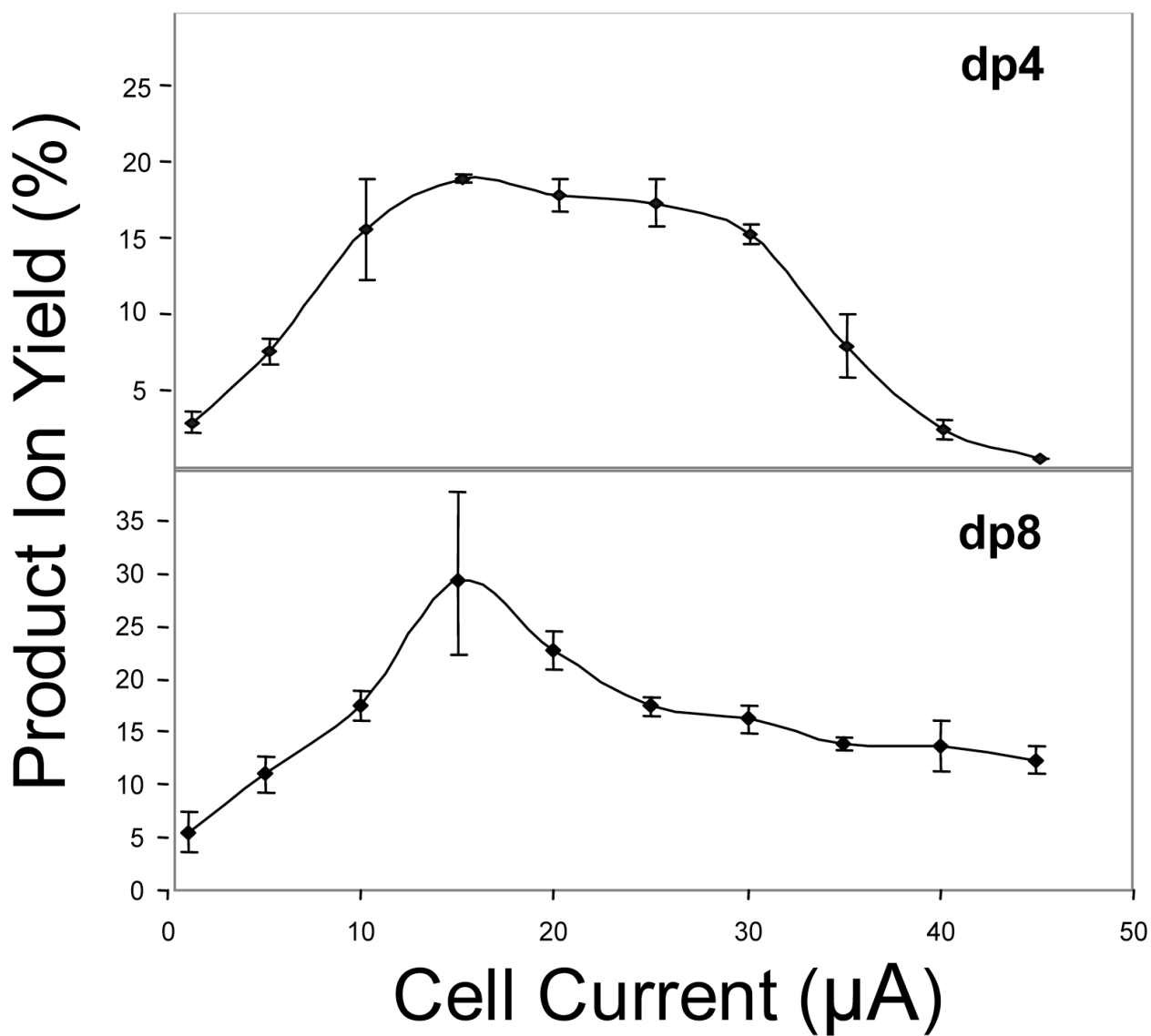
Figure 3. Efficiencies of product formation versus electron current for dermatan sulfate dp4 and dp8 at a heater current of 1.6A, showing a maximum at 15 \mu A.
