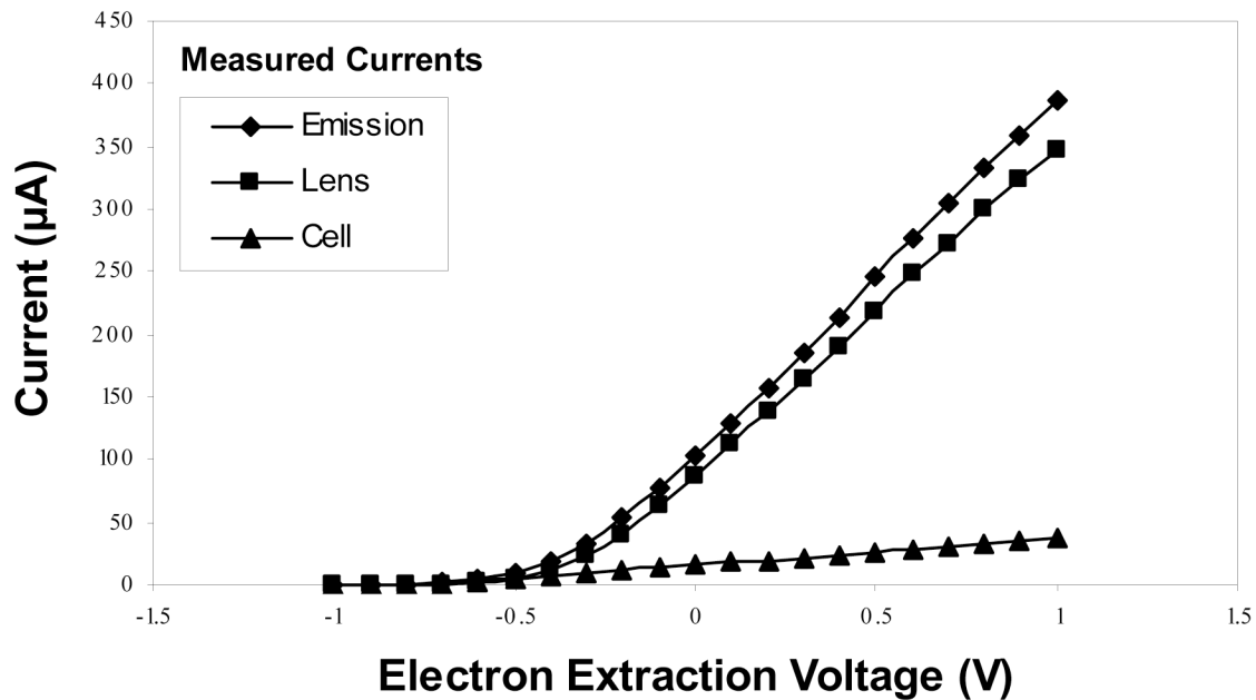
Figure 2. Electron currents ( \mu\text{A} ) as a function of the potential difference between the extraction lens and dispenser cathode, \Delta V , at a heater current of 1.6A. A sub-optimal transmission efficiency is observed for electrons entering the FTICR analyzer cell.
