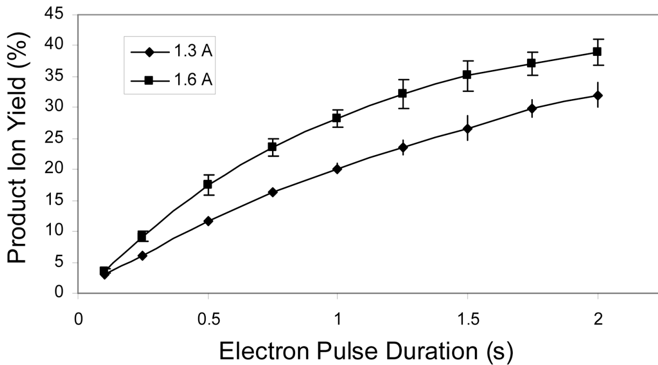
Figure 6. Efficiency of product formation as a function of electron pulse duration at heater currents of 1.3 A and 1.6 A.
