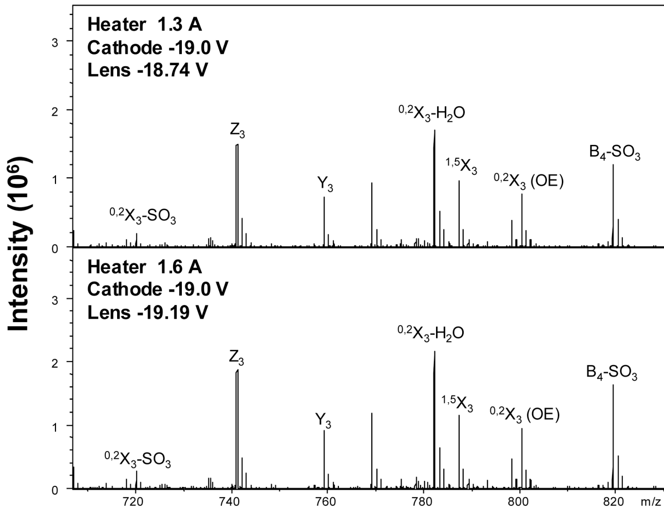
Figure 5. EDD mass spectra acquired at heater current settings of 1.3 A and 1.6 A showing identical fragmentation obtained by adjusting the electron extraction voltage.
