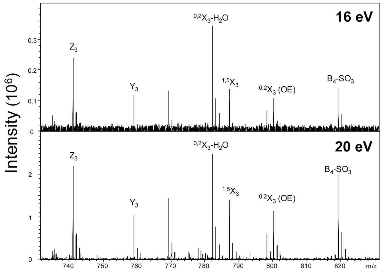
Figure 8. EDD mass spectra obtained at 16 eV and 20 eV showing similar product ion distributions.
