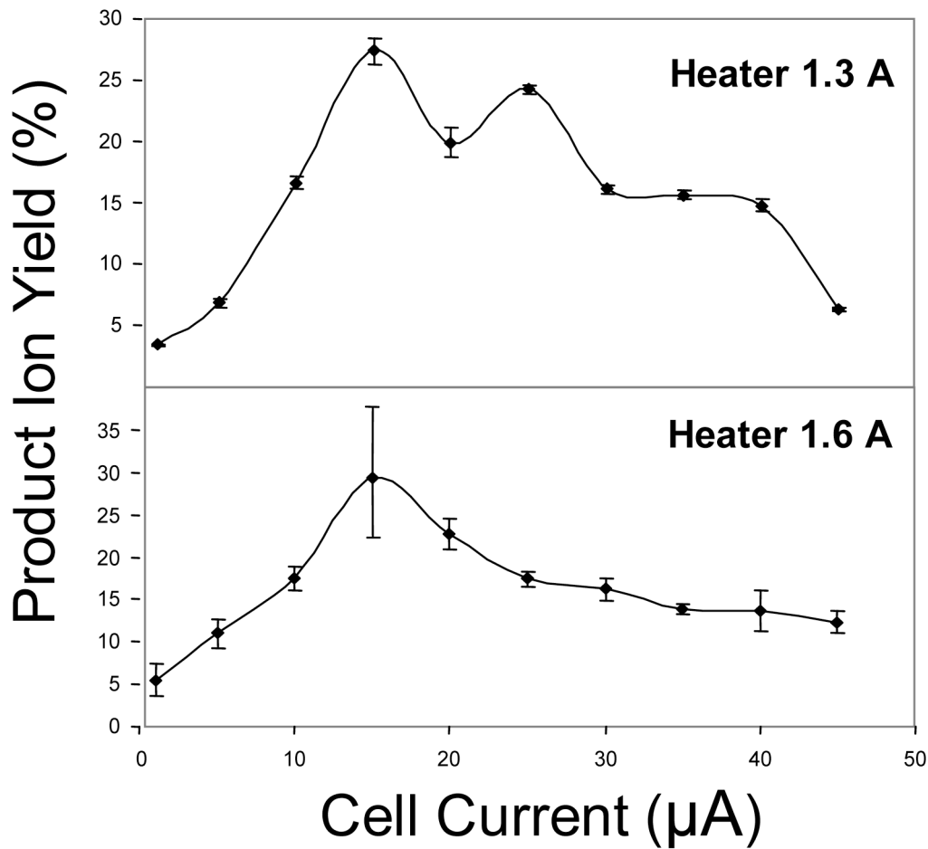
Figure 4. Efficiency of product formation for dermatan sulfate dp8 as a function of cell current at heater currents of 1.3A and 1.6A.
