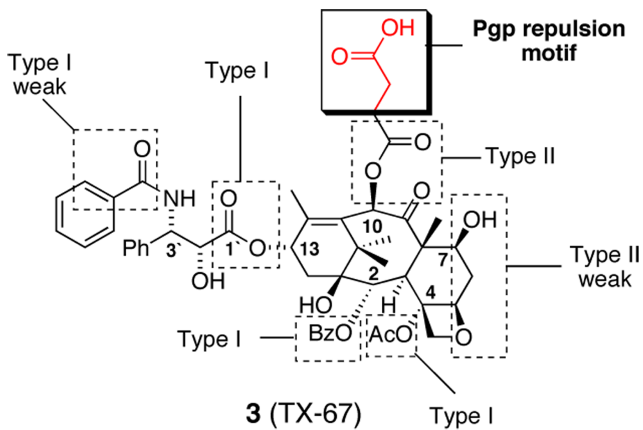
Figure 2. TX-67 recognition and repulsion elements.
