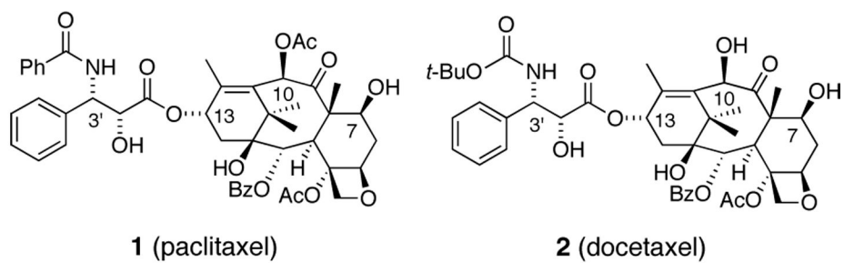
Figure 1. Paclitaxel and docetaxel
