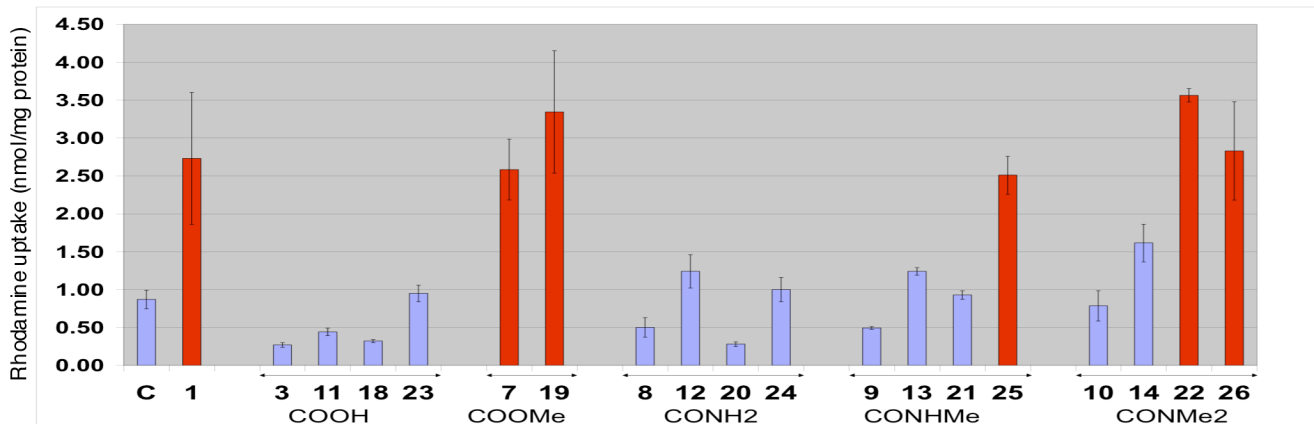
Figure 3. Rhodamine uptake results for compounds 1 (paclitaxel), C10 and C7 acids ( 3 , 11 , 18 and 23 ), C10 and C7 esters ( 7 and 19 ), C10 and C7 primary amides ( 8 , 12 , 20 and 24 ), C10 and C7 secondary amides ( 9 , 13 , 21 , and 25 ), and C10 and C7 tertiary amides ( 10 , 14 , 22 , and 26 ) in BMEC's. Paclitaxel and the derivatives were present at a concentration of 10 \mu M. The concentration of rhodamine was 5 \mu M. C = control. Compounds that significantly increase rhodamine 123 uptake are shown as red bars. Compounds causing decreased or limited rhodamine 123 uptake are shown in blue.
