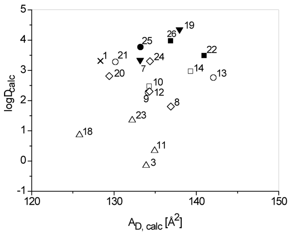
Figure 4. Calculations of cross-sectional areas, A_D and \log D values at pH 7.4 for paclitaxel and analogues. X = Paclitaxel, \Delta = \text{CO}_2\text{H} , \nabla = \text{CO}_2\text{Me} , \diamond = \text{CONH}_2 , \circ = \text{CONHMe} , \bullet = \text{CONHMe} , \square = \text{CONMe}_2 , \blacksquare \text{CONMe}_2 (filled symbols = Pgp substrates).
