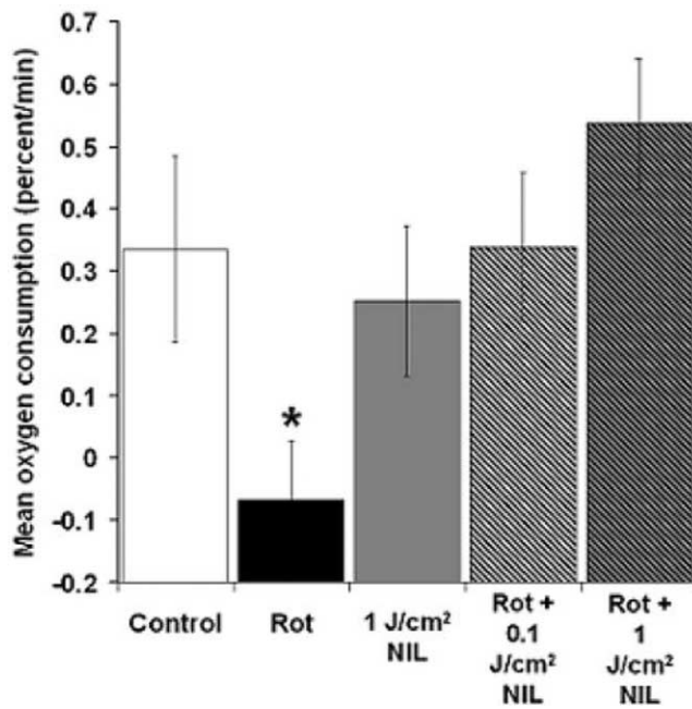
Figure 10. Effect of near-infrared light on cell respiration in vitro . Rotenone decreased the rate of oxygen consumption. Small ( 0.1 \text{ J/cm}^2 ) and large ( 1 \text{ J/cm}^2 ) pulses of NIL reversed the inhibitory effect of rotenone. Rot, Rotenone ( 10 \mu\text{M} ). Significant difference compared with control at *p < 0.05 .
