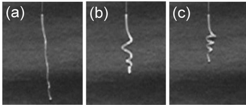
Fig. 1. (a) to (c) Series of images showing a cylindrical SMP rod ( 380\ \mu\text{m} diameter) attached to a 100\text{-}\mu\text{m} -core optical fiber undergoing thermally induced shape recovery from a secondary straight form to its programmed coil form. The SMP was doped with a laser-absorbing dye to enable laser heating. The SMP diffusers could be similarly programmed to change shape if desired. An IR diode laser was used as the actuation source.
