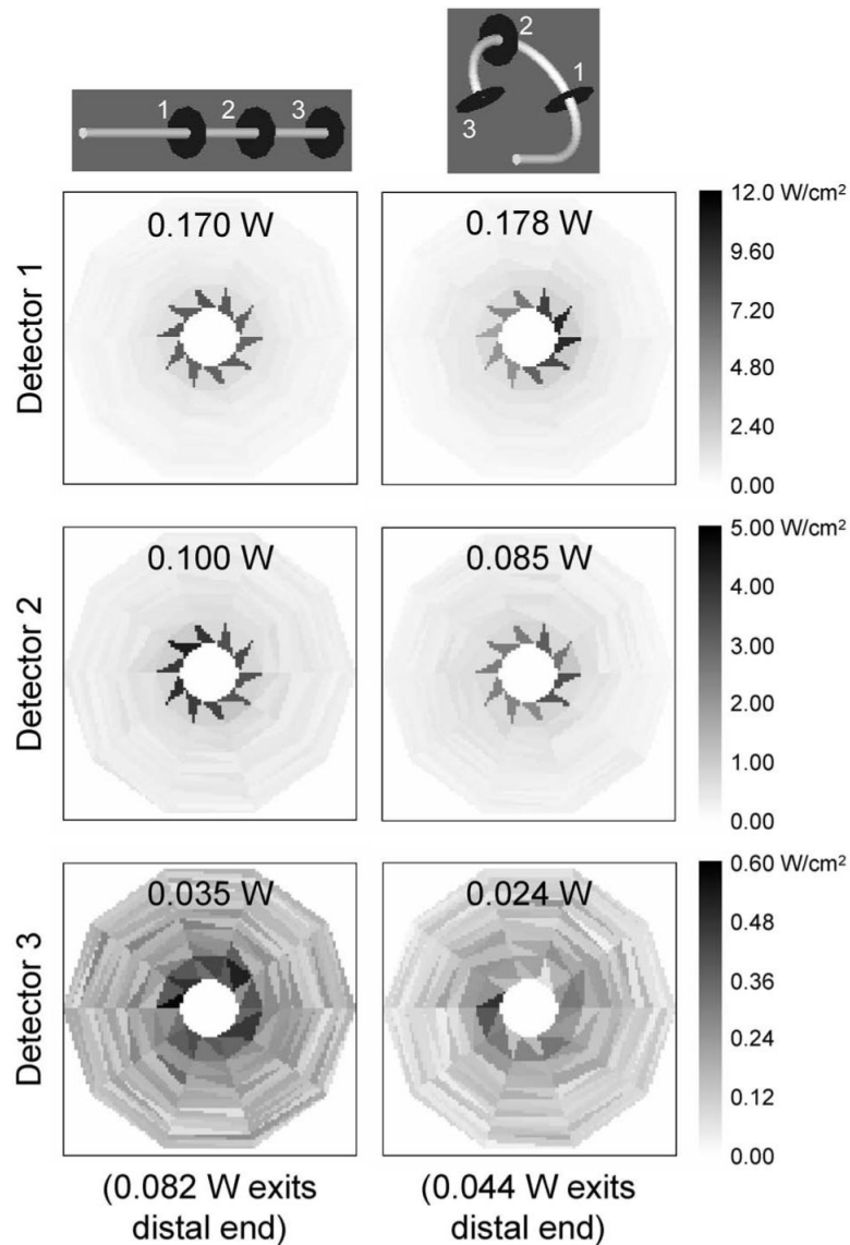
Fig. 7. ZEMAX simulation comparing the emission of straight (left column) and curved (right column) 1-mm-diam, 3-cm-long diffusers. The radius of curvature of the curved diffuser is 6.366 mm and the bend angle is 270 deg. A total power of 1 W was launched from the embedded fiber. The irradiance at the surface of each of the three virtual annular detectors is plotted and the total incident power is noted for each diffuser. The power exiting the distal end of each diffuser is also noted. The detector surfaces are comprised of triangular pixels.
