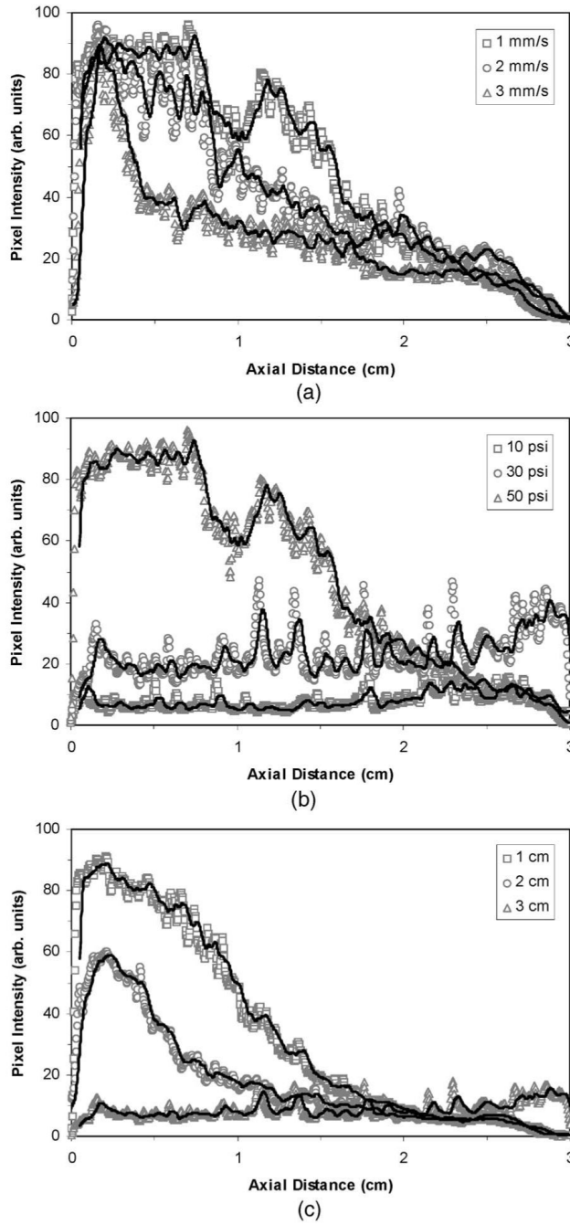
Fig. 4. Selected axial emission profiles illustrating the effect of changing the (a) nozzle translation speed, (b) blasting pressure, and (c) nozzle-to-sample distance for the 1-mm-diam diffusers. In (a), the nozzle-to-sample distance was 3 cm and the blasting pressure was 50 psi. In (b), the nozzle-to-sample distance was 3 cm and the nozzle translation speed was 1 mm/s. In (c), the nozzle translation speed was 1 mm/s and the blasting pressure was 30 psi. The curves were normalized based on the amount of light emitted over the entire 3-cm length, measured using the integrating sphere system.
