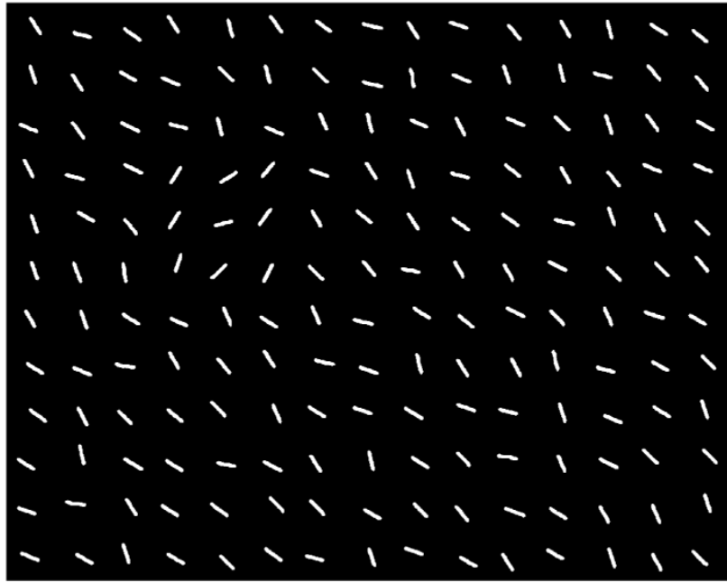
Fig. 5. Sample of the texture display used in Experiment 3. To limit performance, variability is introduced in the line elements' orientation (average orientation is \pm 45^\circ from vertical). A 3 \times 3 target patch is visible in the upper left quadrant of the display.
