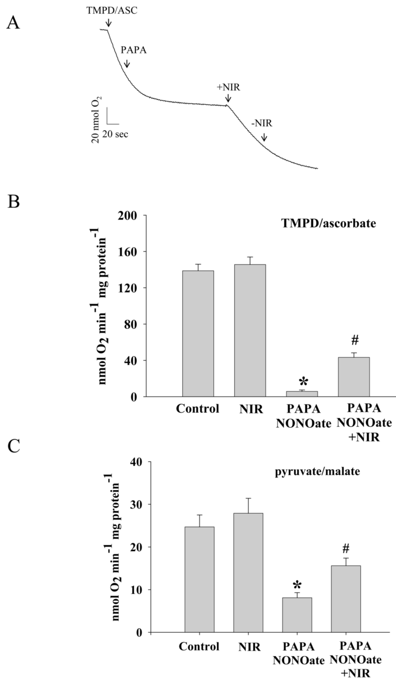
Figure 7. NO-induced inhibition of oxygen consumption is reversed by NIR
