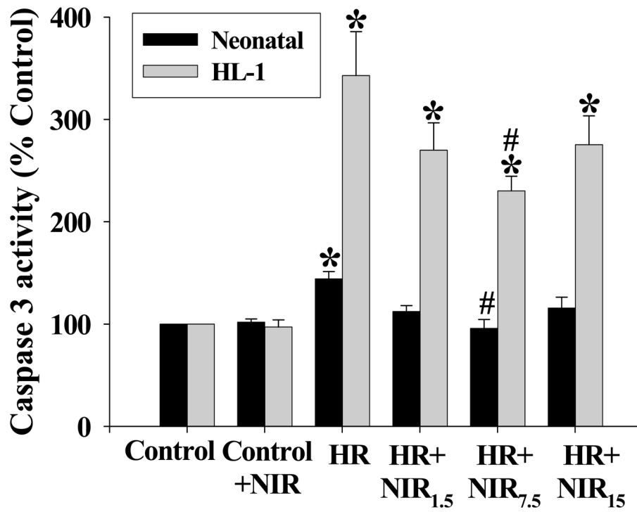
Figure 2. NIR reverses HR-induced increase in caspase-3 activity Neonatal myocytes and HL-1 cells were subjected to normoxia (Control) or HR with or without treatment with NIR (1.5, 7.5, and 15 J/cm 2 ). Caspase-3 activity was measured using specific caspase substrate AcDEVD-pNA as described under Materials and Methods. Values of the absorption were expressed as % of control which was set as 100%. * p < 0.01 vs. control, # p < 0.01 vs. HR, n=6.
