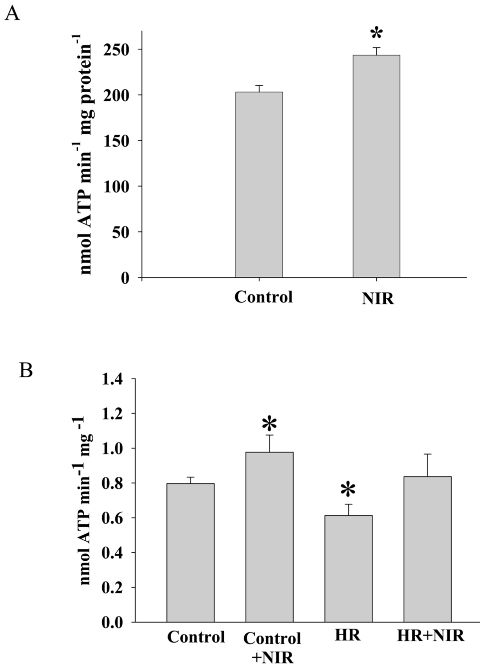
Figure 8. NIR exposure increased mitochondrial ATP synthesis
