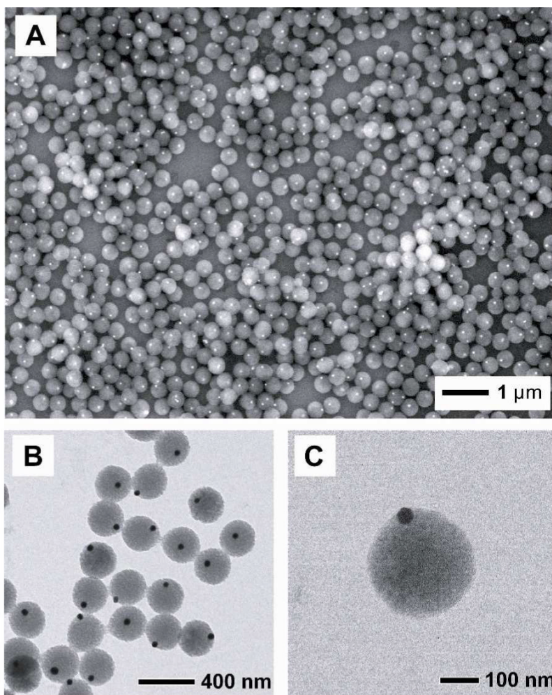
Figure 1. (A) SEM and (B, C) TEM images of the Au-PS asymmetric particles. The average diameter of the Au nanoparticles and the PS beads were 50 and 300 nm, respectively.
