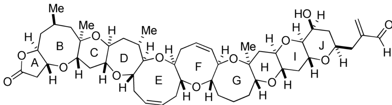
brevetoxin A
