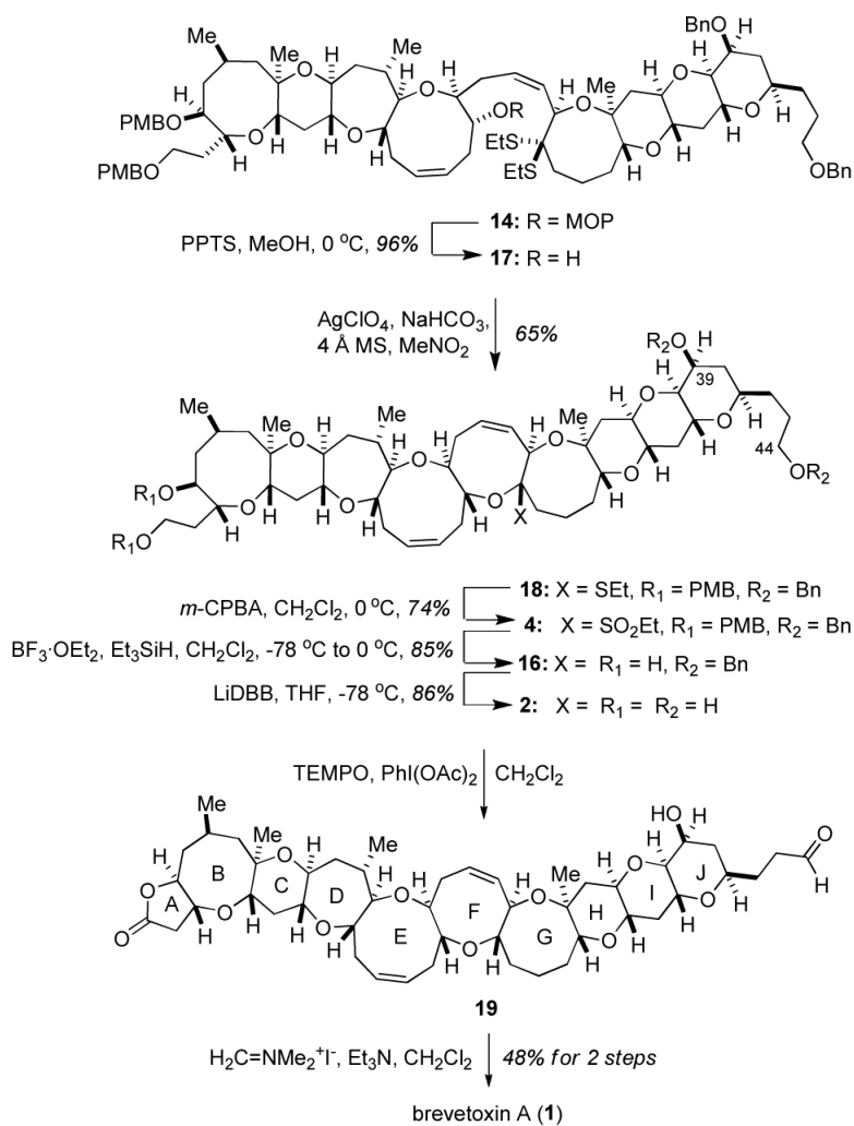
Scheme 5. Completion of Brevetoxin A ( \mathbf{1} ) a
