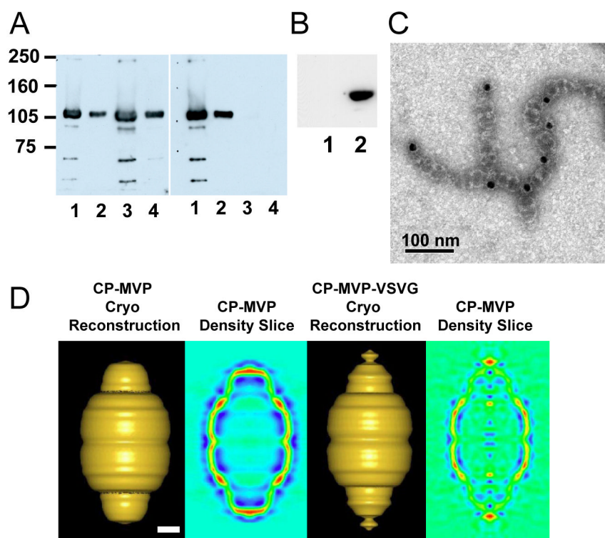
Figure 1. The C-terminal peptide tag is located on the exterior of the caps of recombinant vaults A. Western blot analysis comparing purified CP-MVP-VSVG (lanes 1 and 2) and CP-MVP (lanes 3 and 4) recombinant vaults to confirm the presence of the VSVG peptide tag. Lanes 1 and 3 represent vaults purified from the 40% sucrose gradient layers and lanes 2 and 4 are from the 45% sucrose gradient layer. The left panel was probed with an anti-MVP polyclonal antibody and the right panel was probed with an anti-VSVG monoclonal antibody. Protein standards are indicated. B. S20 extracts from CP-MVP-VSVG infected Sf9 cells were immunoprecipitated with either anti-T7 (lane 1) or anti-VSVG (lane 2) monoclonal antibodies complexed with protein G sepharose, proteins bound to the washed beads were analyzed by Western blotting with an anti-MVP polyclonal antibody. C. Electron micrograph of uranyl acetate-stained CP-MVP-VSVG vaults incubated with anti-VSVG monoclonal antibody followed by 15 nm gold labeled anti-mouse IgG. D. Comparison of cryoEM single-particle reconstructions of CP-MVP 31 and CP-MVP-VSVG recombinant vaults. Surface views and vertical density slices through the reconstructions are shown with both reconstructions filtered to 38 Å resolution. In the slices the strongest density is in red and the weakest in blue. Scale bar, 100 Å.
