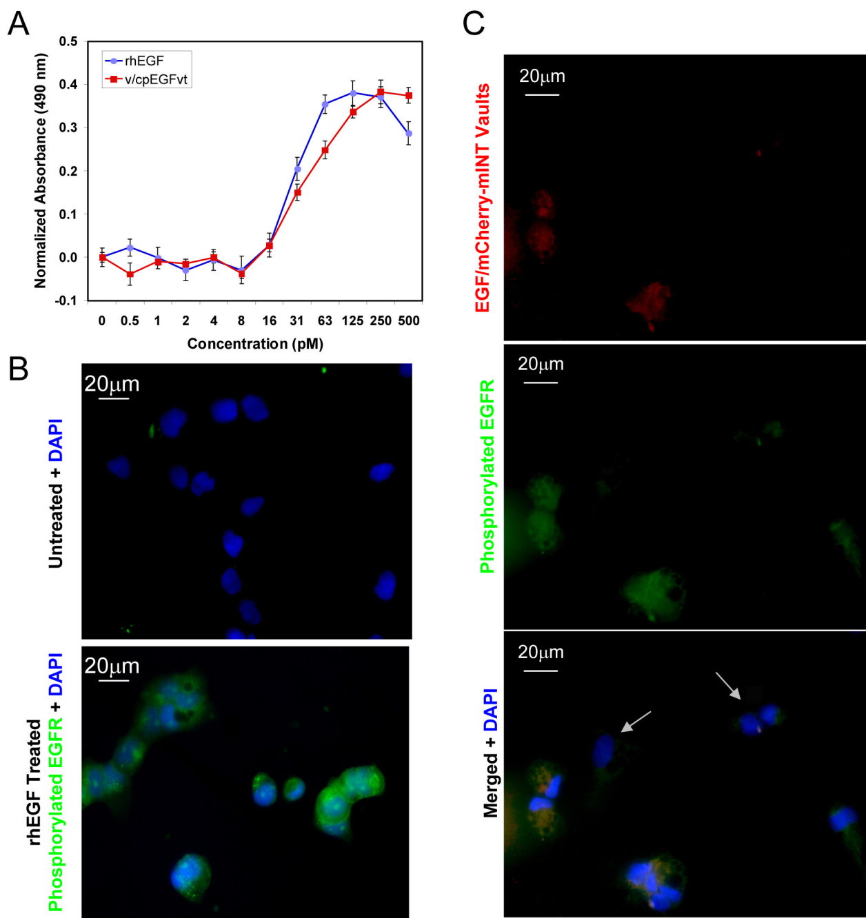
Figure 6. EGF vaults are bioactive
