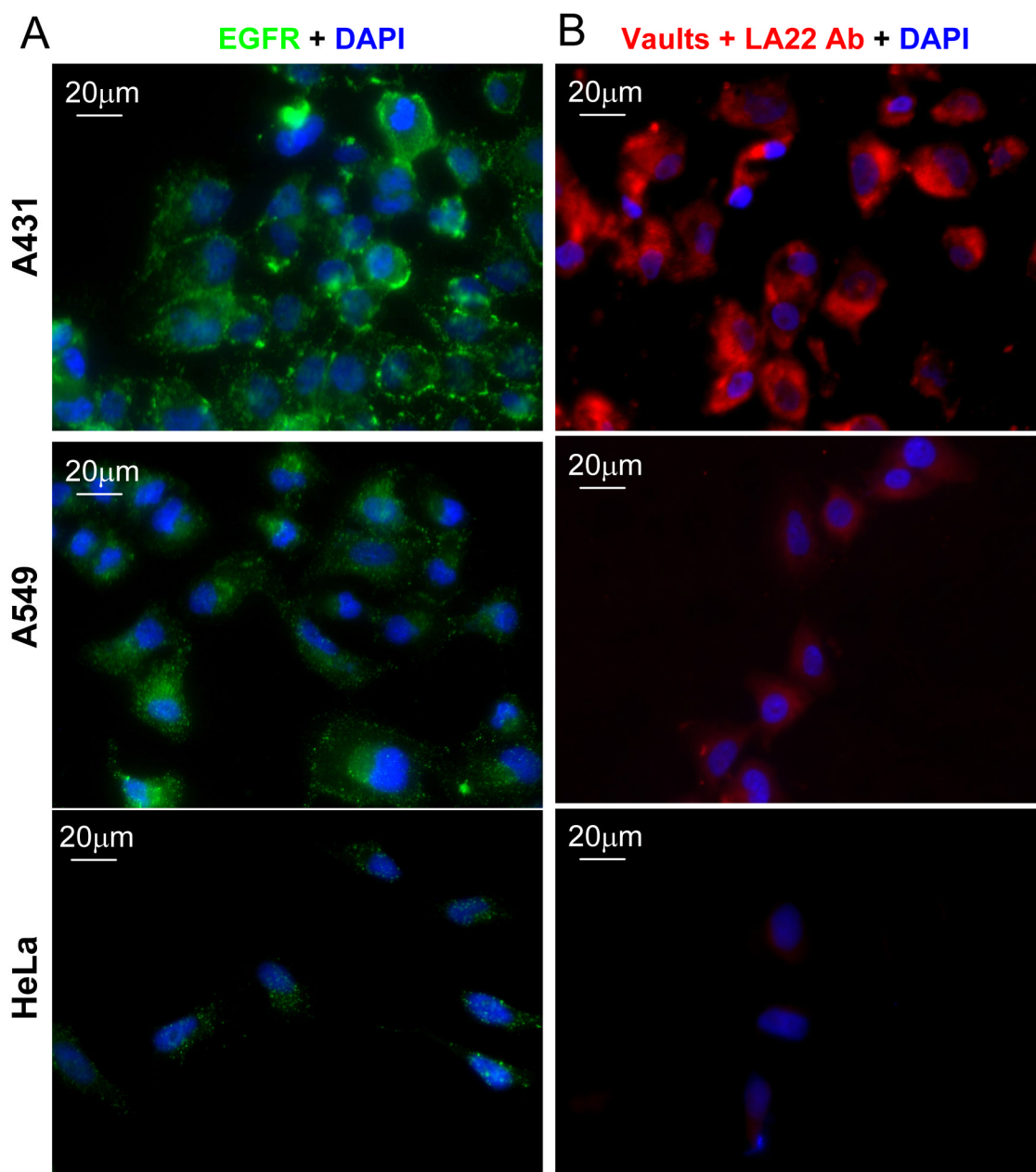
Figure 4. Antibody-mediated binding of vaults to EGFR
