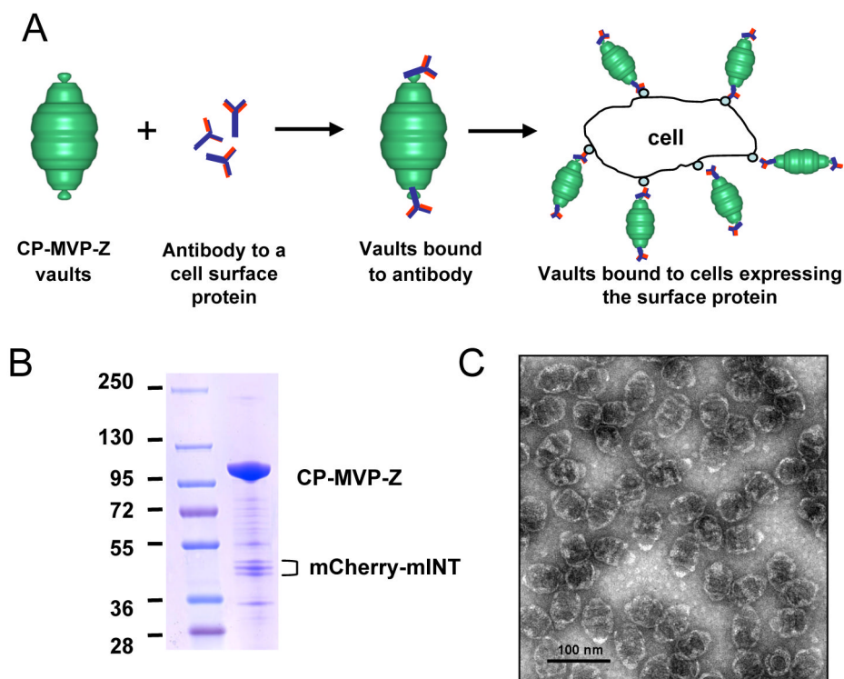
Figure 3. Model for antibody-mediated targeting of vaults
