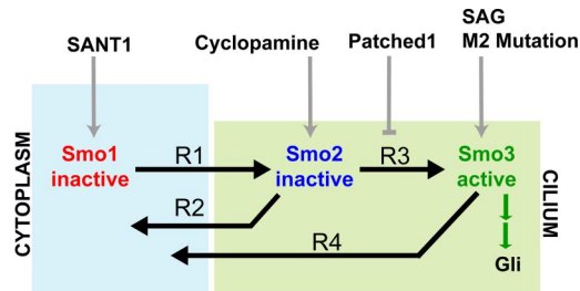
Fig. 5. Full activation of Smo requires ciliary transport coupled to a second activation step. Full activation of cytoplasmic Smo (Smo1) first requires its transport to cilia (Smo2), followed by a second, rate-controlling activation step in cilia that converts Smo2 to Smo3, the state capable of engaging downstream signaling machinery that ultimately leads to activation of the Gli proteins. Solid black arrows denote the individual steps. Transport to cilia (Smo1→Smo2) is controlled by entry and exit steps, designated R1 and R2; the activation step (Smo2→Smo3) is controlled by R3; and the exit of Smo3 from cilia is controlled by R4. The proposed site of action of various regulators of Hh signaling regulators is denoted above the kinetic scheme by light gray arrows.
