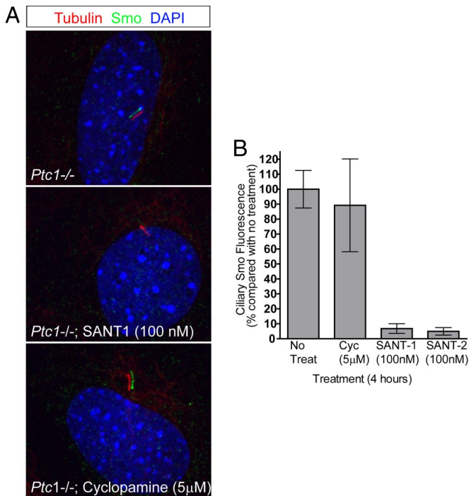
Fig. 3. Constitutive Smo accumulation in the cilia of Ptc1 -/- cells can be reversed with SANTS1 and 2, but not with cyclopamine. MEFs from Ptc1 -/- mice were treated with SANTI1, SANTI2, or cyclopamine for 4 h and then stained with DAPI to show nuclei (blue), anti-Smo (green), or anti-acetylated tubulin (red). (A) Shifted overlays of confocal images of Ptc1 -/- cells treated as indicated. (B) The mean ( \pm SEM) Smo fluorescence at cilia under the indicated conditions, calculated based on images of the type shown in (A).
