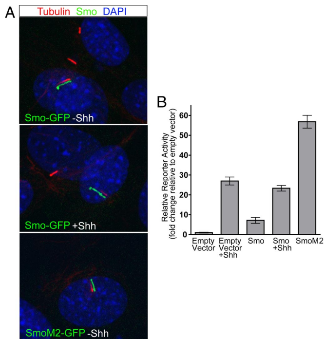
Fig. 1. Smo localization in cilia is not sufficient to activate Hh target genes. Smo-GFP (with or without Shh) and SmoM2-GFP transfected into NIH 3T3 cells accumulate in cilia to similar degrees (A); however, SmoM2-GFP is a substantially better inducer of a Gli-responsive transcriptional reporter (B). (A) Single-plane confocal images of NIH 3T3 cells transfected with the indicated constructs show the ciliary marker acetylated tubulin (red) detected by immunofluorescence, Smo-GFP (green) detected by GFP fluorescence, and nuclei (blue) detected by DAPI staining. All 3 channels are shown as a single overlay, with the green (Smo) layer shifted relative to the other channels (shifted overlay) for easier visualization. (B) NIH 3T3 cells were cotransfected with a Gli-luciferase transcriptional reporter and either an empty vector control or the same Smo constructs as used in (A). The mean ( \pm SEM) luciferase reporter activity was measured after treatment with or without Shh for 24 h.
