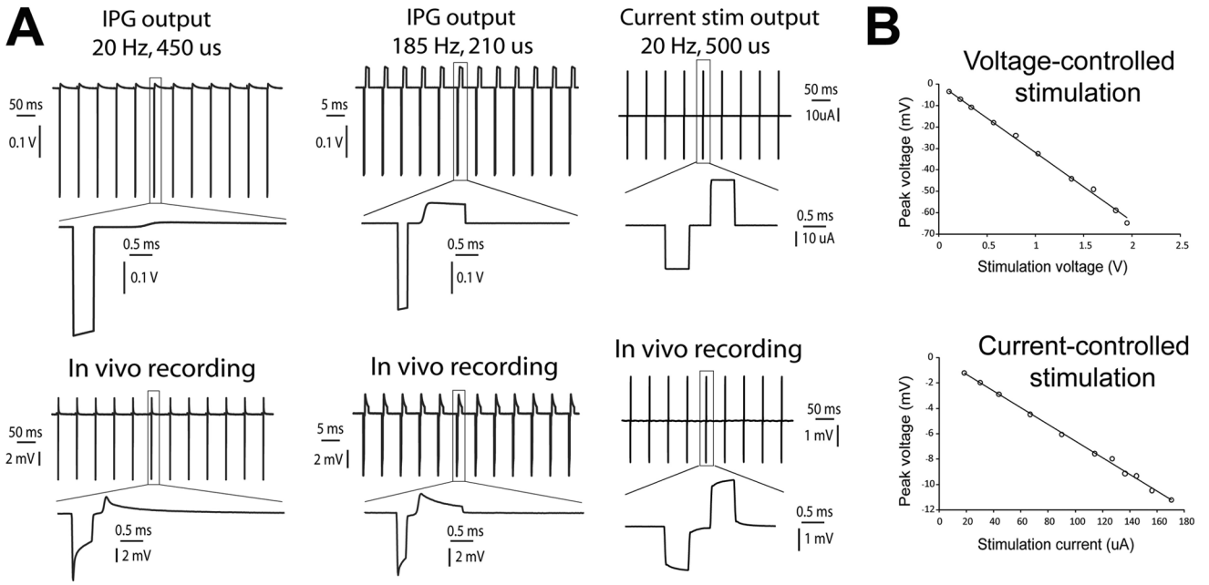
Figure 3. In vivo stimulus waveform recordings. A. Voltage-controlled (IPG) and current-controlled stimulus waveforms at 20 Hz and 185 Hz recorded across a 1 k \Omega resistor (top) and corresponding voltage responses recorded in vivo (bottom). B. The peak voltage recorded in vivo was proportional to the applied stimulus amplitude for both voltage-controlled and current-controlled stimulation.
