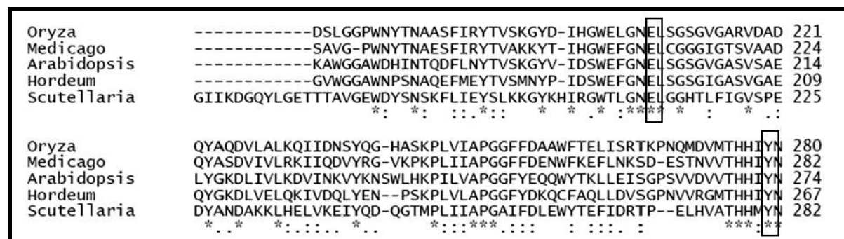
Figure 1: A segment of the multiple sequence alignment of plant heparanase from Oryza sativa , Medicago truncatula , Arabidopsis thaliana , Hordeum vulgare and Scutellaria baicalensis is shown. The conserved catalytic site residues (glutamic acid and tyrosine) are shown in boxes.
