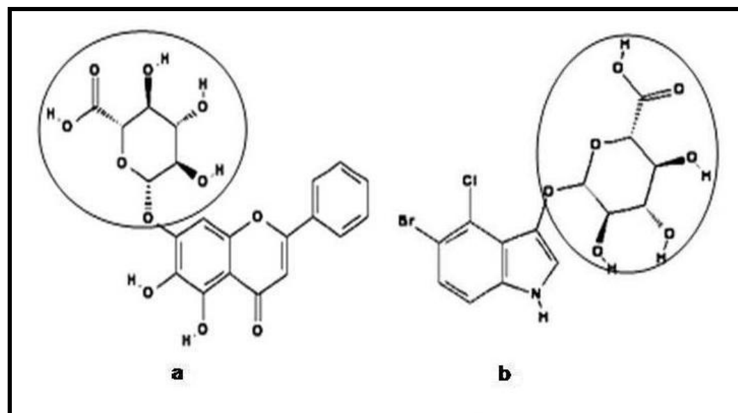
Figure 2: Structure of (a) Baicalein 7-O- \beta -D-glucuronide and (b) X-Gluc showing the glucuronate moiety present in common (encircled).
