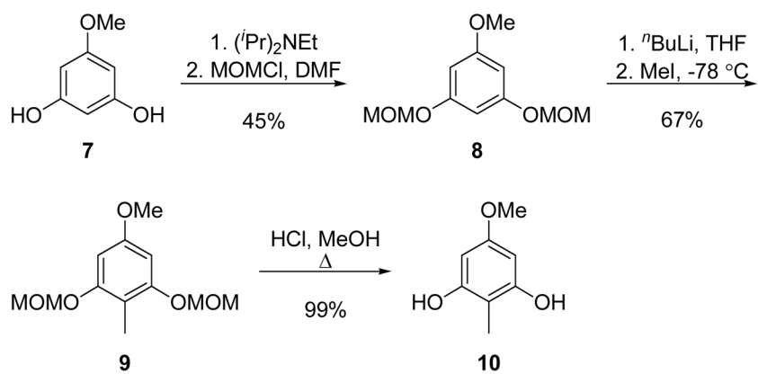
Scheme 3. Synthesis of 5-substituted resorcinol.
