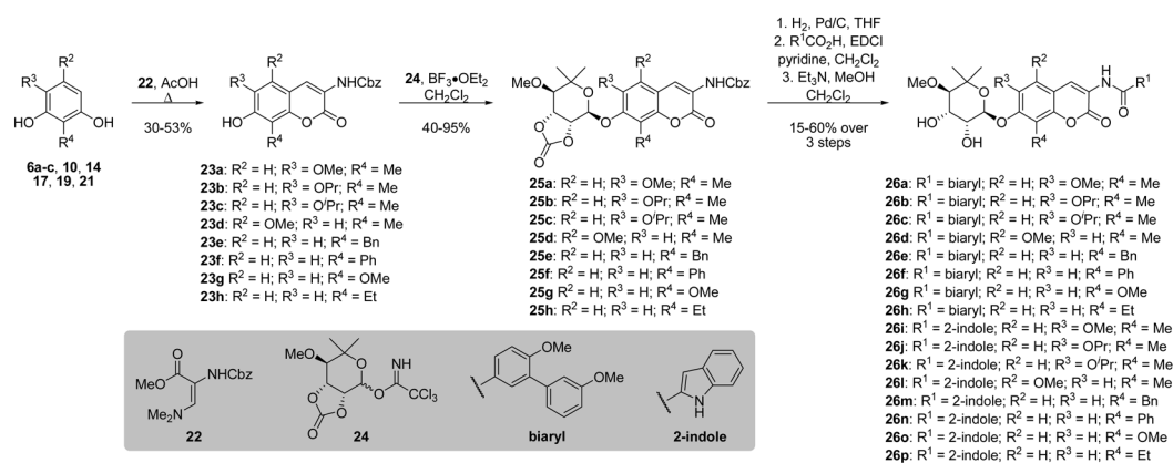
Scheme 6. Preparation of 5-, 6-, and 8-modified novobiocin analogues.
