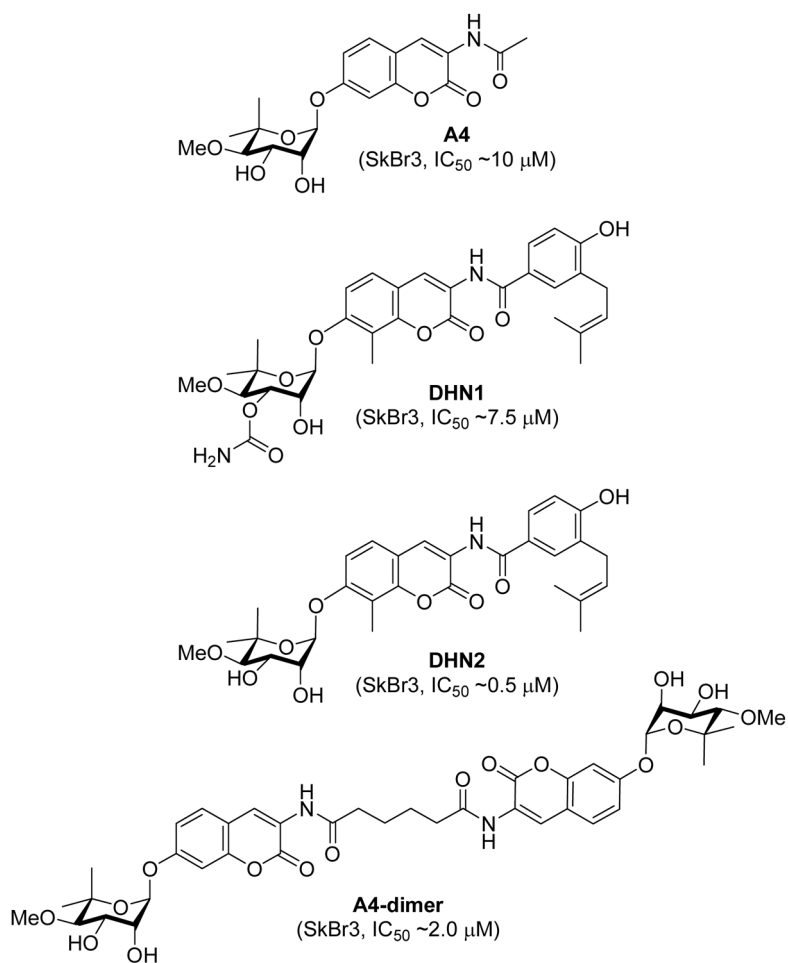
Figure 2. Structures of A4 , DHN1 , DHN2 , and A4 dimer .
