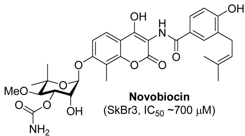
Figure 1. Structure of novobiocin.
