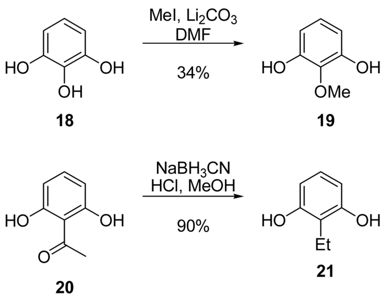
Scheme 5. Synthesis of 2-methoxy resorcinol and 2-ethyl resorcinol.
