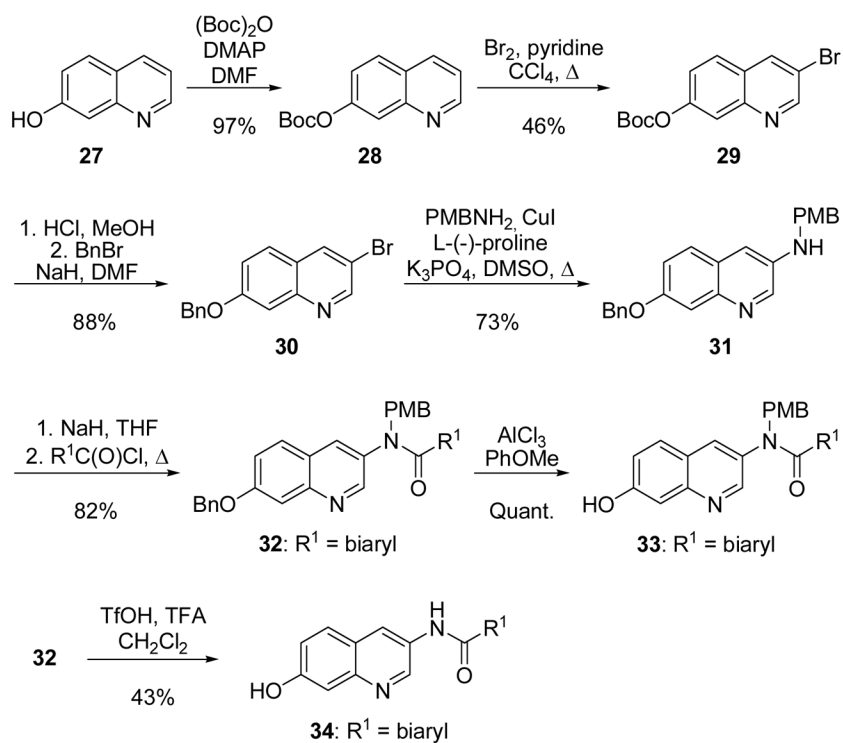
Scheme 7. Syntheses of 7-hydroxyquinolines.
