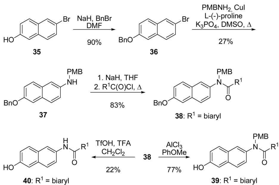
Scheme 8. Syntheses of 6-hydroxynaphthalenes.
