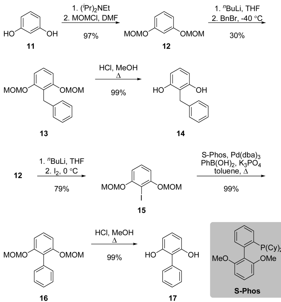
Scheme 4. Syntheses of 2-substituted resorcinols.
