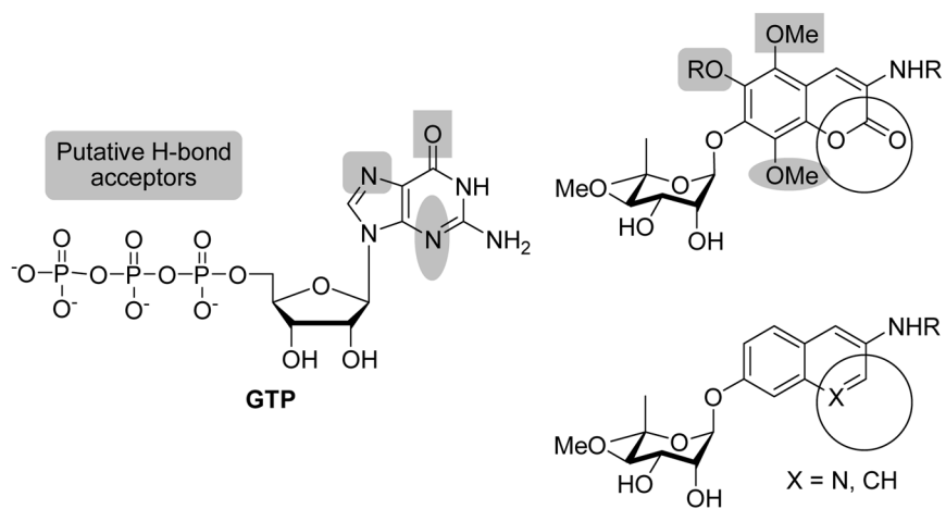
Figure 3. Complementarity of GTP and coumarin analogues.
