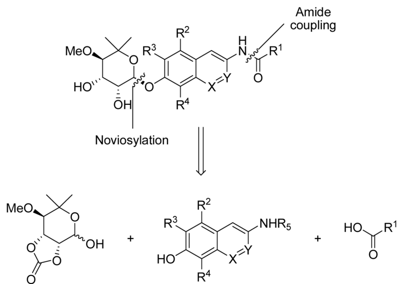
Scheme 1. Retrosynthesis of novobiocin analogues.
