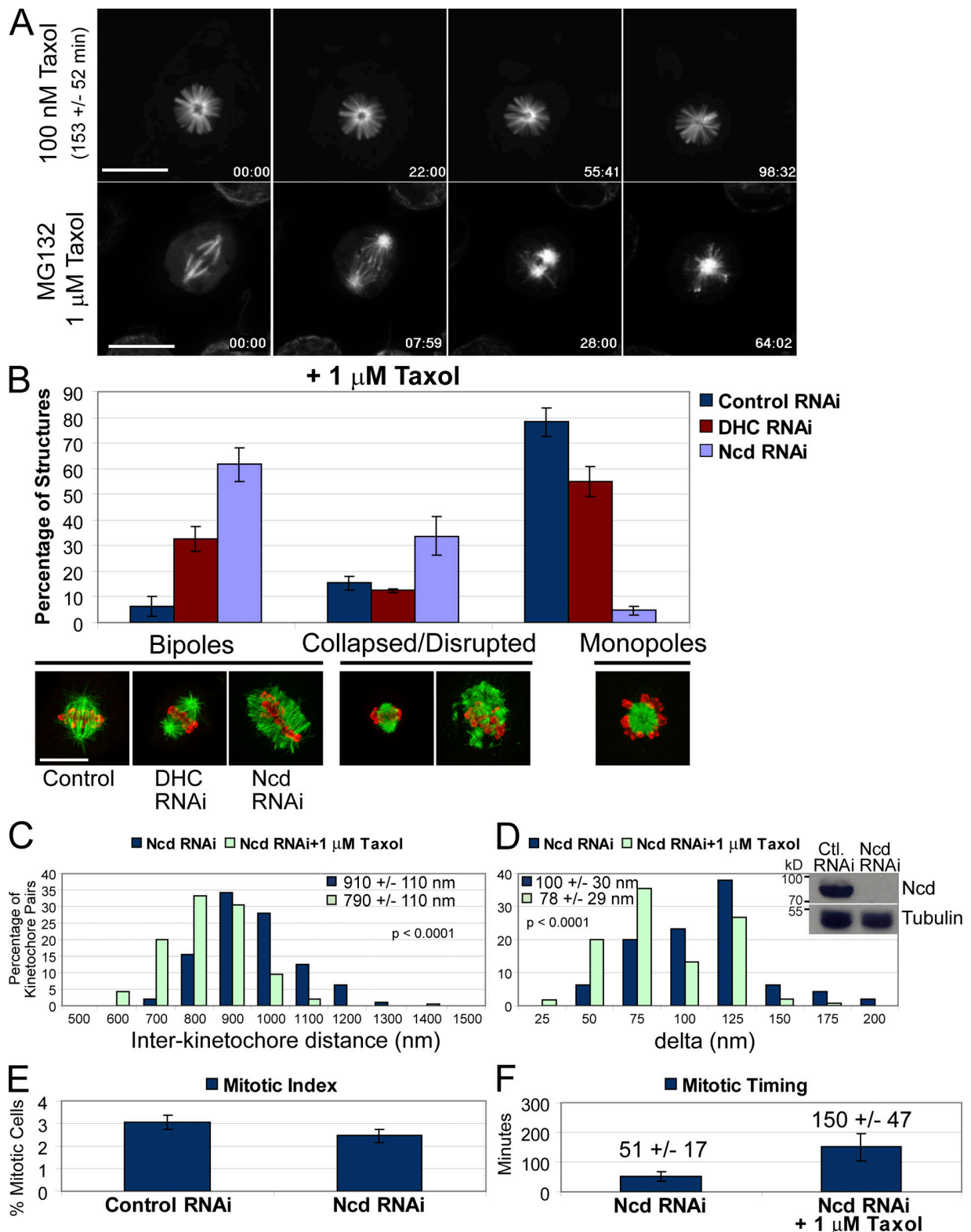
Figure 3. Treatment with 1 \mu M taxol reduces delta and activates the SAC. (A) Selected frames from time-lapse imaging of a preformed taxol monopole (top) and an MG132-treated bipolar spindle collapsing into a monopole after the addition of 1 \mu M taxol (bottom). Taxol monopoles delay in mitosis for 153 \pm 52 min. (B) Taxol-induced spindle collapse is mediated by minus end-directed motor activity. The graph shows the percentage of each indicated structure with representative images after treatment with 1 \mu M taxol for 1 h. (C and D) Treatment of Ncd RNAi structures with 1 \mu M taxol ( n = 240 kinetochore pairs) causes a reduction in both the interkinetochore distance and delta relative to Ncd RNAi alone ( n = 95 kinetochore pairs). Ncd is undetectable by Western blotting (inset) after dsRNA treatment (96 h). (E) Ncd RNAi does not cause an increase in the number of mitotic cells in a cycling population. (F) Ncd RNAi cells divide with normal kinetics (51 \pm 17 min; n = 100 cells), but addition of 1 \mu M taxol delays them in mitosis for 150 \pm 47 min ( n = 77 cells), indicating that the SAC is activated. The mean values \pm standard deviations and the two-tailed p -values are shown in each graph. Error bars represent the standard deviations. Bars, 10 \mu m.
