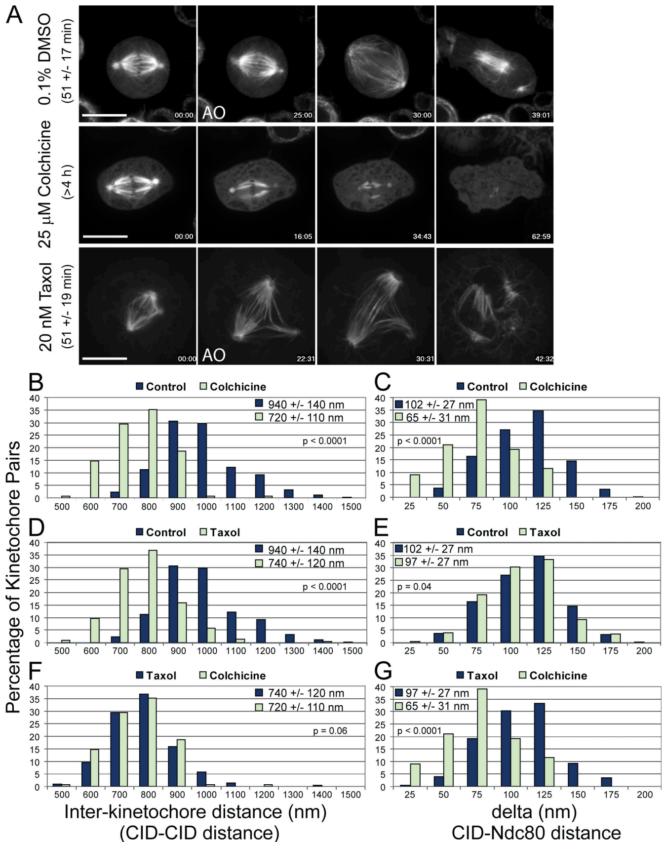
Figure 2. Microtubule poisons differentially affect interkinetochore distance and delta. (A) Selected frames from time-lapse imaging of GFP-tubulin-expressing S2 cells after treatment with DMSO, 25 \mu M colchicine, or 20 nM taxol. DMSO control cells progress through mitosis (as defined by chromosome condensation to anaphase onset [AO]) in 51 \pm 17 min ( n = 124 cells). Spindle microtubules completely depolymerize within 1 h after the addition of 25 \mu M
