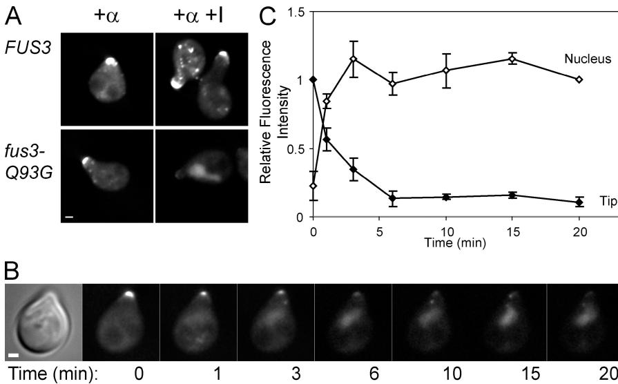
Figure 4. Fus3p activity is required to maintain Fus2p in the cytoplasm. (A) FUS3 (MY10011) or FUS3-Q93G (MY10012) strains were pregrown in selective medium and induced with \alpha factor for 90 min. Cells were placed on an agarose slide containing \alpha factor with or without 1-NA-PP1, a selective inhibitor of Fus3p-Q93G (Matheos et al., 2004), and examined microscopically. (B) The fus3-Q93G strain (MY10012) was grown as in A and placed in a microscope flow cell chamber. Inhibitor was added at t = 0 , and images were collected at 1-min intervals. (C) GFP fluorescence in the nucleus and at the shmoo tip was measured in 11 cells treated as in B and expressed as a fraction of t = 20 min (nucleus) or t = 0 (tip). Closed symbols, relative shmoo tip fluorescence; open symbols, relative nuclear fluorescence (see Materials and methods). Error bars represent \pm SEM. Bars, 1 \mu m.
