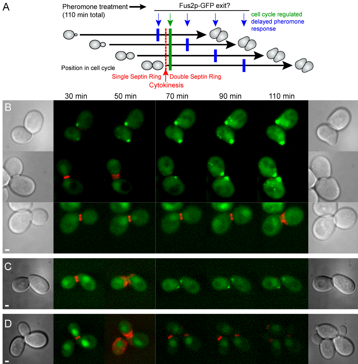
Figure 1. Fus2p is expressed in pheromone-treated cells before cytokinesis but remains in the nucleus until after cell division. (A) Experiment schematic. An asynchronous cell population expressing Fus2p-GFP and Cdc3-mCherryFP, an indicator of cytokinesis (red), was treated with pheromone for 110 min (black arrows) and examined microscopically over time. If Fus2p-GFP nuclear exit is solely dependent on pheromone signaling, exit should occur at similar times after exposure for all cells (blue arrows). If Fus2p-GFP nuclear exit requires completion of the previous cell cycle, exit should occur soon after cytokinesis independent of the length of pheromone signaling (green arrow). (B) Fus2p-GFP expressed under its own promoter. Strain MY10176 containing FUS2::GFP 104 and CDC3-mCherry was pregrown in selective medium, and \alpha factor was added at t = 0 . Representative cells are shown in which cytokinesis occurred before 30 min, between 30 and 50 min, and between 90 and 110 min (top, middle, and bottom, respectively). (C) Fus2p-GFP expressed under the GAL1 promoter. Strain MY10177 containing P GAL1 -FUS2::GFP 104 and CDC3-mCherry was pregrown in selective medium with galactose; \alpha factor and glucose were added at t = 0 . (D) Pheromone is required for Fus2p-GFP exit G1. MY10177 was examined as in C except that no \alpha factor was added. Bars, 1 \mu m.
