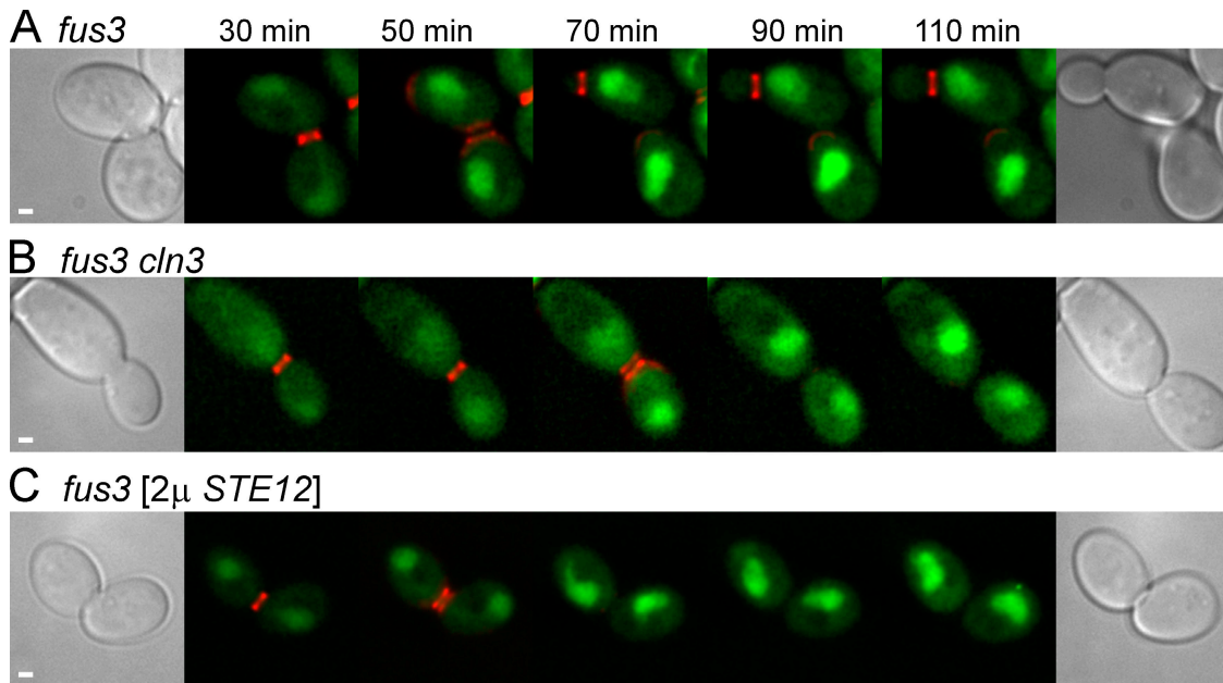
Figure 3. Fus3p is required for Fus2p nuclear exit. (A–C) Fus2p-GFP localization was examined in fus3 (MY10318; A), fus3 cln3 (MY10319; B), and fus3 [2 \mu STE12 ] (MY10322; C) as described in Fig. 1 B. Similar results were obtained when Fus2p-GFP was expressed from the GAL1 promoter. Bars, 1 \mu m.
