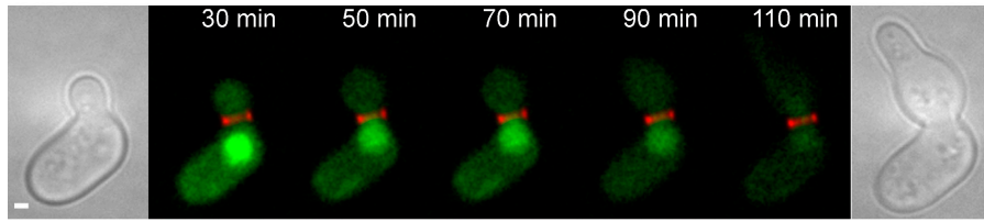
Figure 7. Cdc28p inhibits Fus2p-GFP nuclear exit in G2/M. Localization of GAL1 -expressed Fus2p-GFP was examined as described in Fig. 1 D in cdc28-as1 (MY10324). (A) Cdc28p-as1 inhibitor was added without \alpha factor. (B) Cdc28p-as1 inhibitor and \alpha factor were added together. The images show cytoplasmic and cortical localization in large-budded cells before cytokinesis. The bottom panel shows a cell dying during the course of the experiment. Similar results were obtained when Fus2p-GFP was expressed under its own promoter. Bars, 1 \mu m.
