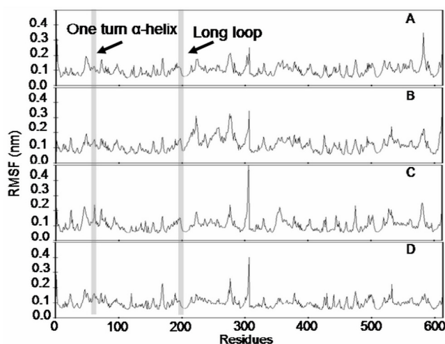
Figure 5 The RMSF with respect to amino acid residues of the SARS CoVMpro. The values were calculated averaging at time range 500–2000 ps of MD simulation. The values of the SARS CoVMpro complexed with octapeptide P3Lys, P3Arg and P3Ile were shown in A, B and C, respectively. The value of the SARS CoVMpro free form was shown in D. The shadow region from left to right represent the region of protein chain namely one turn \alpha -helix (residues 47–54) and long loop (residues 184–192) of SARS CoVMpro, respectively.
