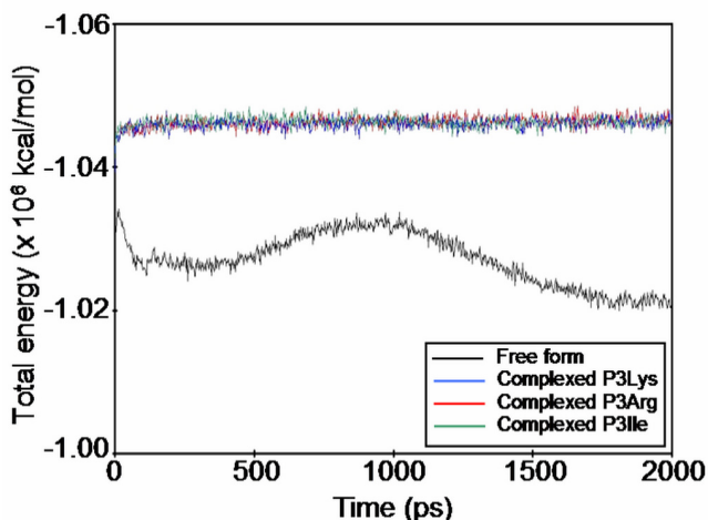
Figure 3 Time dependence of the total energy from MD simulation. The lines of the SARS CoVMpro free form, complexed with octapeptide P3Lys, P3Arg and P3Ile were colored in black, blue, red and green, respectively.
