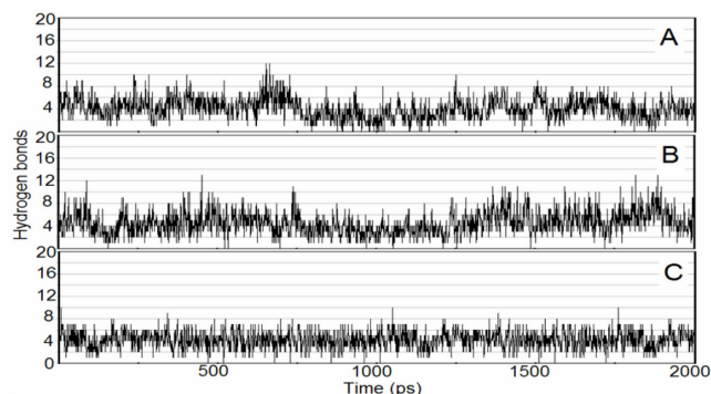
Figure 6 Hydrogen bonds number between the SARS CoVMpro and the octapeptide. The octapeptide P3Lys, P3Arg and P3Ile were shown in A, B and C, respectively.
