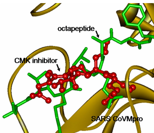
Figure 2 Molecular docking of the octapeptide substrate. The docking performed through superimposition between the hexapeptide chloromethyl ketone inhibitor (red ball and stick) and the octapeptide (green stick).
