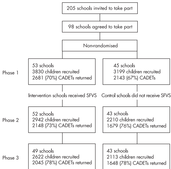
Figure 1 Flow diagram of schools and children recruited, and number of CADETs returned. CADET, child and diet evaluation tool; SFVS, school fruit and vegetable scheme.
