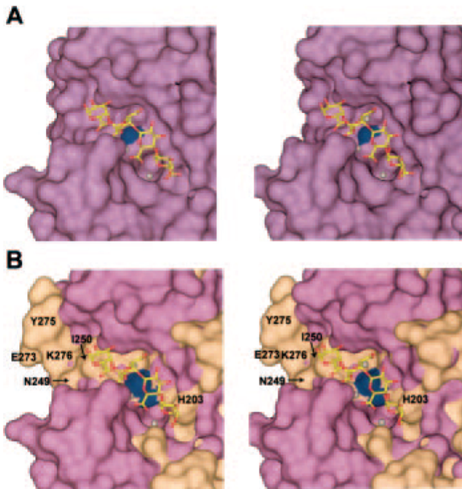
FIG. 6. The surfaces of Jun a 1 ( wheat ) aligned with the R218K mutant of Pel C ( violet ) according to the secondary structural elements
