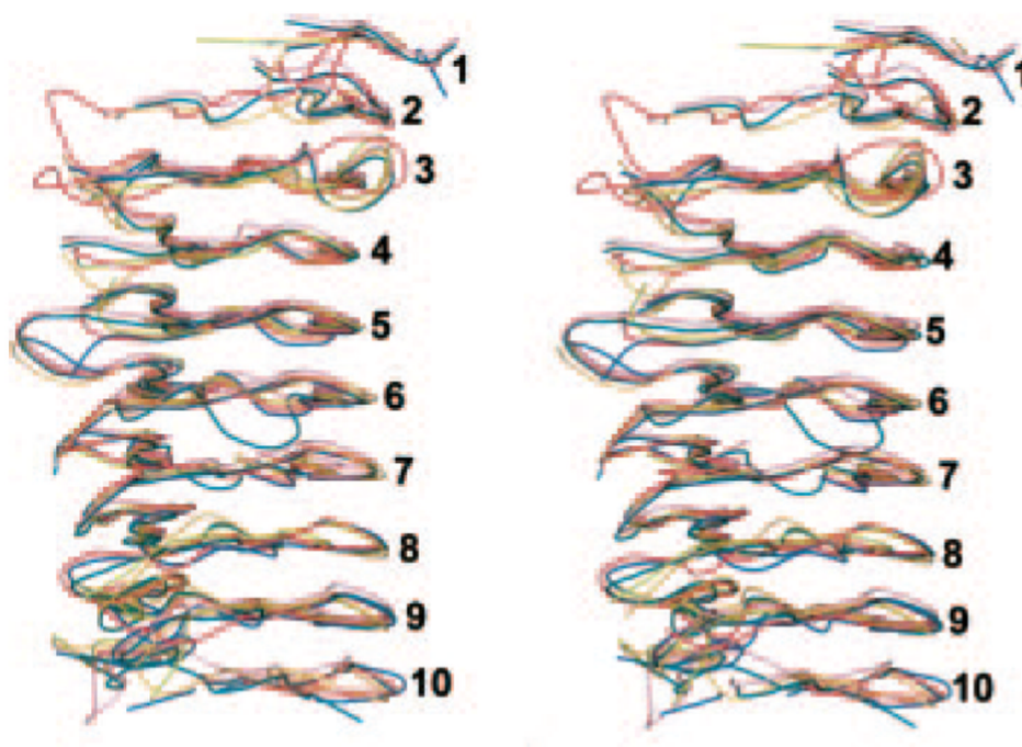
FIG. 2. Stereo view showing similarity of the \beta -helical cores of Jun a 1 (red) and Pnl A (turquoise), Pnl B (magenta), Pel A (orange), Pel C (marine), and B. subtilis Pel (olive) The Pels and Pnls are superimposed on the Jun a 1 by their secondary structural elements. Numbers refer to the PB sheet strand from the N ( top ) to C ( bottom ) termini. Orientation is similar to that of Fig. 1B.
