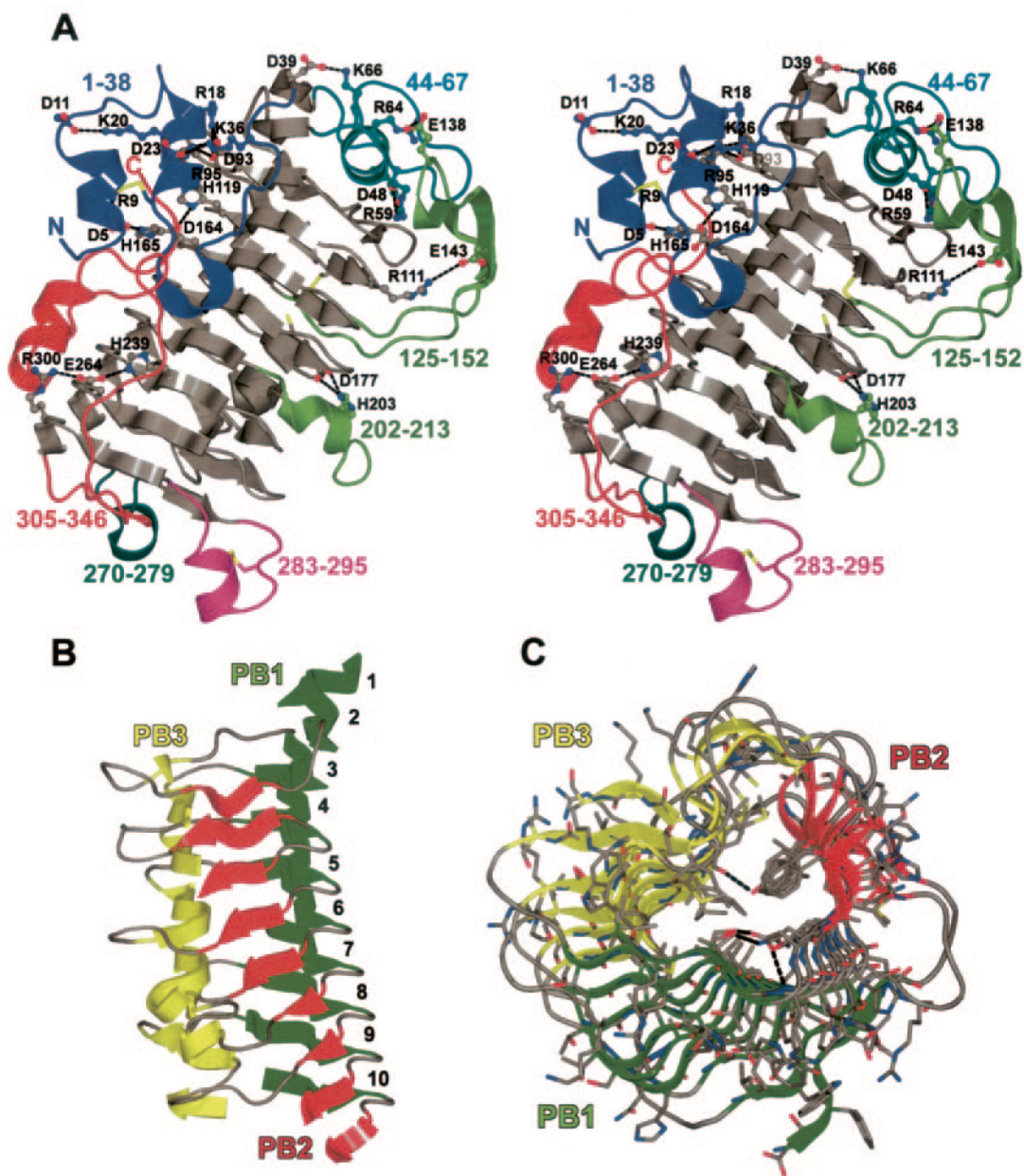
FIG. 1. Structure of Jun a 1
