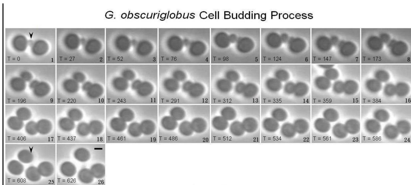
Figure 1 Time-lapse phase contrast micrographs showing G. obscuriglobus budding cell division. Bud initiates from the polar end of the mother cell, grows until it reaches the same size as the mother cell and finally separates from the mother cell. The full budding process takes over 10 hours and approximately 12 hours. Arrowhead indicates the bud at the initiation (frame 1) and after separation (frame 25). Unit of the time in each frame is minutes. Bar – 1 \mu m.
