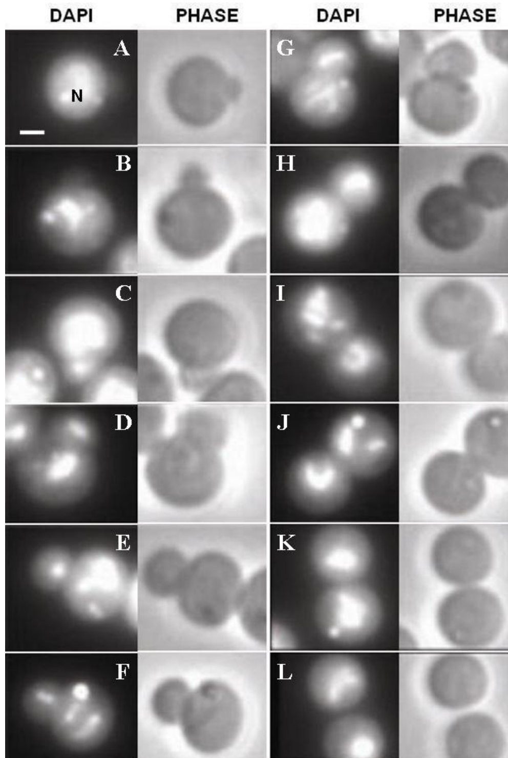
Figure 2 Fluorescence and phase contrast micrographs of individual G. obscuriglobus budding cells. Each pair of micrographs (DAPI and PHASE) represents a different budding stage seen after staining with DAPI and visualizing via fluorescence and phase contrast microscopy, and each letter A-L refers to a paired micrograph (DAPI-stained on the left and PHASE microscopy on the right) of a different cell in each case. Nucleoid (N) DNA is stained with DAPI. Pair A represents the earliest budding stage while pair L represents the final stage. Bar – 1 \mu m.
