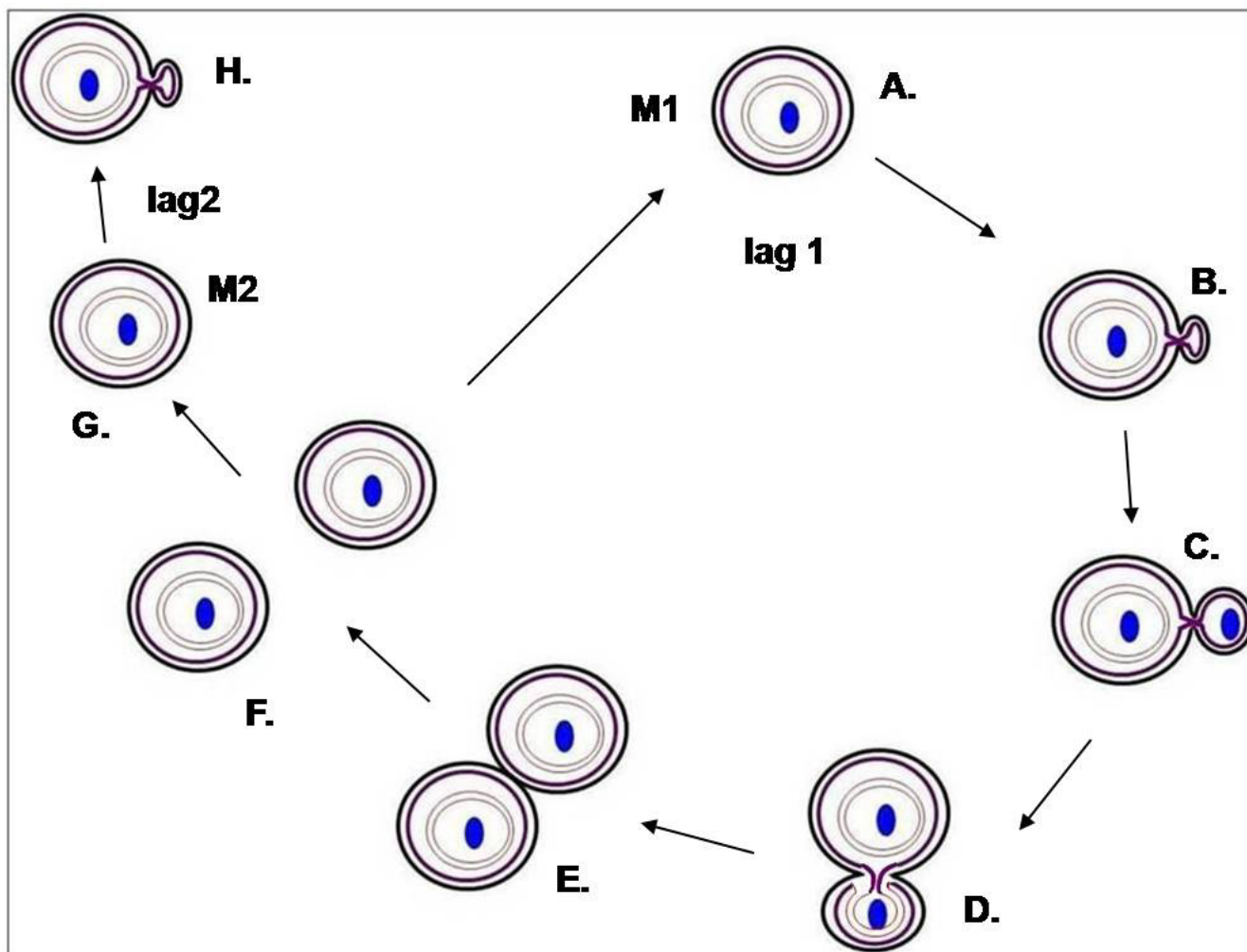
Figure 6 Gemmata obscuriglobus cell budding cycle. In (A) and (B), a bud initiates from one point of the mother cell M1 enclosing a nucleoid (blue) surrounded by a double-membrane nucleoid envelope (grey). The mother cell ICM (dark purple) is continuous with that of the bud (also dark purple). In (C), the naked nucleoid is translocated into the bud at some early budding stage. In (D), the bud nucleoid is surrounded by two membranes where an inner membrane (light purple) continuous with mother cell ICM, and an outer membrane (also light purple) shows continuity with the bud ICM. In (E), the bud nucleoid is completely surrounded by the two closely apposed membranes where membrane fusion and pinching off has resulted in a double-membrane nucleoid envelope completely separated from ICM membranes. (E) is the end-point of a possible model mechanism where the bud reached similar cell size as M1. (F) shows the separation of the mother cell and the matured bud. In (G) and (H), the mother cell M1 can initiate the next budding cycle after a 2–4 hour lag (lag 1) while the matured bud M2 can begin its first budding cycle after a 3–5.5 hour lag (lag2).
