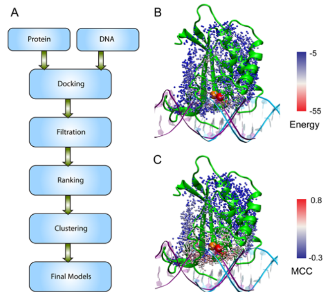
Figure 1. Methodology overview. (A) Flowchart of the DNA-protein complex modeling process. (B–C) An example, Epstein-Barr nuclear antigen-1, illustrates sites that specific-DNA recognition sites on a DNA-binding protein are energetically favorable interaction sites for nonspecific DNA. A nonspecific DNA (cyan) composed of 16 dA·dT base pairs was docked to the protein structure (green), which is complexed with a specific DNA molecule (purple) in the native structure (Protein Data Bank (PDB) code 1b3t). Each point represents one of top 2500 energy-ranked docking models. They are placed at the center of mass (COM) of the interfacial protein residues for a given docked pose, and are color scaled according to (B) energy values and (C) Matthews correlation coefficients. The spheres mark the location of the COM of DNA-interaction sites for the top model (red) and the native structure (orange).
