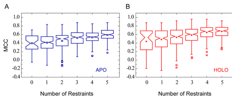
Figure 4. MCC of the Top1 clustering model versus number of geometric restraints applied for model filtration. In each case, up to five native DNA-binding residues were randomly selected as the restraint(s). Models in which the DNA does not contact these restraint residues were discarded, and the remaining models were subjected to clustering. Five independent trials were performed per restraint number per protein. Modeling was performed for both (A) APO and (B) HOLO sets. doi:10.1371/journal.pcbi.1000341.g004
