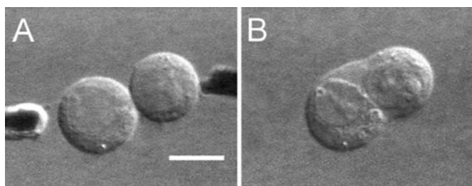
Fig. 2. Creation of a PC-12 homokaryon. The cells were originally located at a distance of about 100 \mu\text{m} from each other. By using the microelectrodes, they were placed next to each other. The cells were pretreated with ac dielectrophoresis (0.3–3 kV/cm, 1 MHz for 1 min), in hypoosmotic sorbitol fusion medium. A shows cells immediately after dielectrophoresis, and a close contact is visualized by the flattened contact zone between the cells. After dielectrophoresis for 30 s, five dc fusion pulses were applied (3 kV/cm, 1-ms duration for each pulse, at approximately 1 Hz), after which an immediate broadening of the contact zone between the cells could be visualized. Within 1 min, a cytoplasmic continuity was observed, and after 2 min, the shape had stabilized, as shown in B . Bar = 10 \mu\text{m} .
