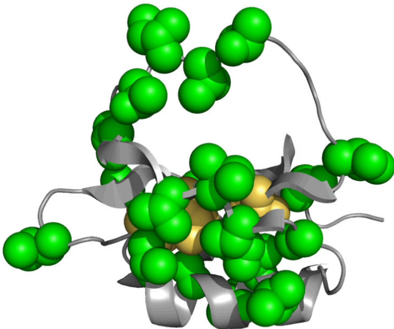
Figure 5. A graphical summary of the ^2\text{H} side-chain dynamics results. In yellow are the sites of the individual single mutants (L68A, L68V, I76V, V66A, V28A). The green residues are those methyl-bearing side chains that have significant changes in S^2_{\text{axis}} in no fewer than 4 of the 5 single mutants investigated. Changes in the amplitude of side-chain motion radiate to all regions of the three dimensional structure and encompass nearly every methyl group which could be experimentally observed.
