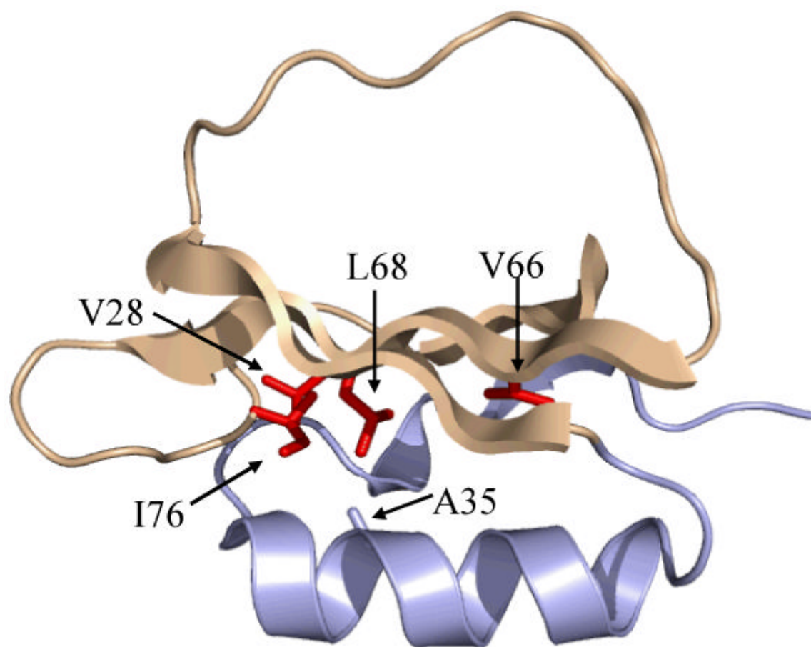
Figure 1. The structure of chymotrypsin inhibitor 2 (PDB code 2CI2), with the sites of mutation examined in this study shown in red. The third canonical member of the CI2 folding nucleus, A35, has not been examined in this work and is shown in gray. The backbone coloring corresponds to the two distinct regions of dynamical perturbation (N-terminal region, light blue; C-terminal region, beige) revealed by ^{15}\text{N} relaxation experiments (see text).
