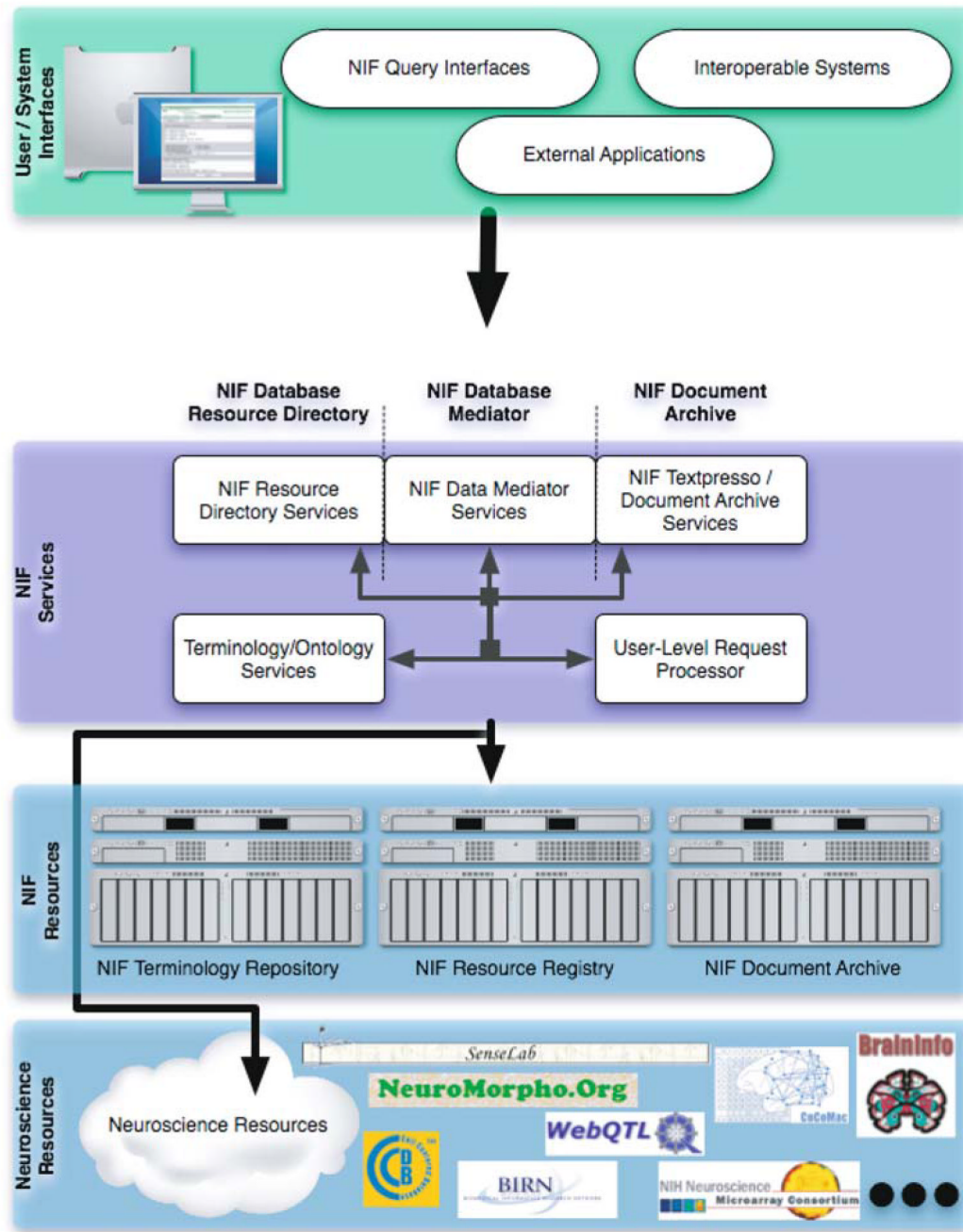
Fig. 4. Overview of the NIFv1 implementation core architecture
