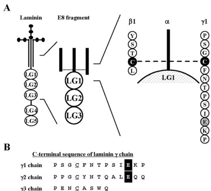
FIGURE 1. Schematic representations of laminin and the C-terminal amino acid sequences of the human laminin \gamma 1, \gamma 2, and \gamma 3 chains. A, schematic diagrams of recombinant laminin, its E8 fragment and the C-terminal amino acid sequences of its \beta 1 and \gamma 1 chains. Cys residues are circled in black, and disulfide bonds are depicted by broken lines. The C-terminal Glu residue of the \gamma 1 chain is shaded. B, C-terminal amino acid sequences of the human laminin \gamma 1, \gamma 2, and \gamma 3 chains. Cys residues are underlined. The black boxes represent the Glu residues conserved between the \gamma 1 and \gamma 2 chains.
