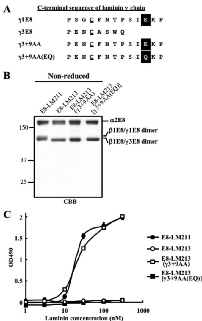
FIGURE 5. Binding of \alpha 7 X 2 \beta 1 integrin to the E8 fragments of laminin-213 mutants. A , C-terminal amino acid sequences of the \gamma 1 and \gamma 3 chains and \gamma 3 mutants with substitutions within the C-terminal tail. The Cys residues are underlined. \gamma 1 E 8 , control E8 fragment of the \gamma 1 chain; \gamma 3 E 8 , E8 fragment of the \gamma 3 chain; \gamma 3 + 9 A A , E8 fragment of the \gamma 3 chain with the C-terminal nine amino acids of the \gamma 1 chain; \gamma 3 + 9 A A (E Q) , \gamma 3 + 9 A A in which the Glu residue (E) is replaced by Gln (Q). The black boxes represent the conserved Glu residues and the substituted Gln residue. B , the E8 fragments of laminin-211 (E8-LM211), laminin-213 (E8-LM213), and the laminin-213 mutant proteins E8-LM213 ( \gamma 3 + 9 A A ) and E8-LM213 ( \gamma 3 + 9 A A (E Q) ) were separated by SDS-PAGE in 12% gels under non-reducing conditions followed by Coomassie Brilliant Blue (CBB) staining. The positions of molecular size markers are shown on the left. C , binding of \alpha 7 X 2 \beta 1 integrin to the E8 fragments of laminin-211, laminin-213, and the laminin-213 mutant proteins. 96-well microtiter plates were coated with increasing concentrations of the E8 fragments of laminin-211, laminin-213, and laminin-213 mutant proteins, blocked with BSA, and incubated with 20 nM \alpha 7 X 2 \beta 1 integrin. The amounts of bound \alpha 7 X 2 \beta 1 integrin were quantified as described under "Experimental Procedures." Each point represents the mean \pm S.D. of triplicate assays.
