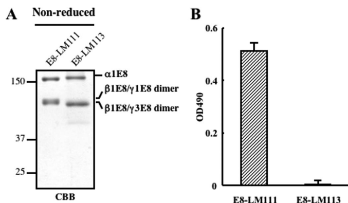
FIGURE 4. Binding of \alpha 6 \beta 1 integrin to the E8 fragment of laminin-113. A , purified E8 fragments of laminin-111 (E8-LM111) and laminin-113 (E8-LM113) were separated by SDS-PAGE in 12% gels under non-reducing conditions followed by Coomassie Brilliant Blue (CBB) staining. The positions of molecular size markers are shown on the left. B , binding of \alpha 6 \beta 1 integrin to the E8 fragments of laminin-111 and laminin-113. 96-well microtiter plates were coated with the E8 fragments of laminin-111 (E8-LM111; positive control) and laminin-113 (E8-LM113) at 100 nM, blocked with BSA, and incubated with 20 nM \alpha 6 \beta 1 integrin. The amounts of bound \alpha 6 \beta 1 integrin were quantified as described under "Experimental Procedures." Each column and bar represents the mean \pm S.D. of triplicate assays, respectively.
