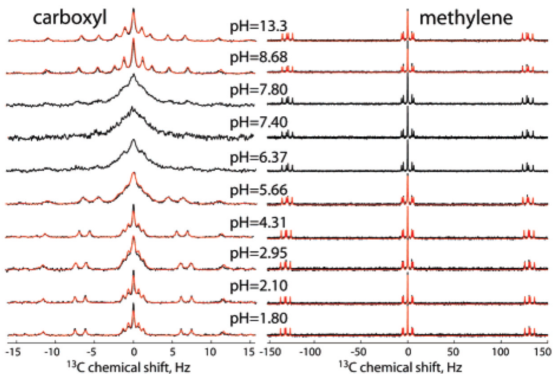
Figure 2. ^{13}\text{C} NMR multiplets (experimental in black and simulated fits in red) of natural abundance succinic acid at various pH. All spectra acquired at 14 T with 128–512 scans using Varian triple resonance H/C/N probe without ^1\text{H} decoupling.
