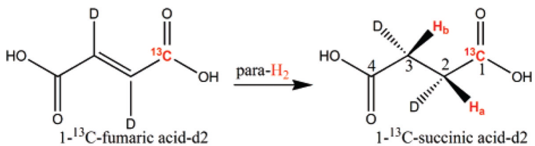
Figure 1. Cis molecular addition of parahydrogen to 1\text{-}^{13}\text{C} -fumaric acid- d_2 to produce 1\text{-}^{13}\text{C} -succinic acid- d_2 . The catalytic reaction was carried out at 62\text{ }^\circ\text{C} in \text{H}_2\text{O} or \text{D}_2\text{O} with substrate concentrations of 1–5 mM.
