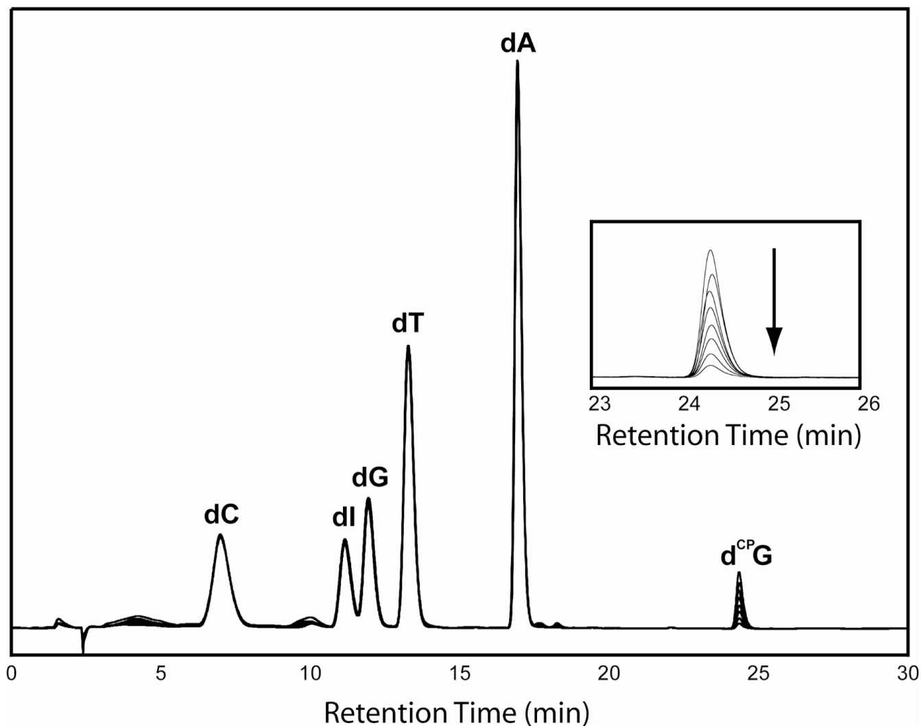
Figure 2. Overlaid HPLC traces at 260 nm for digested nucleosides from AQA 2 irradiated at 350 nm for 0, 1, 2, 3, 5, 7, 10, and 15 min. Traces are normalized to the height of the dT peak, and the inset demonstrates that the peak corresponding to d CP G steadily degrades with respect to increased irradiation time. Conditions are as described in Experimental.
