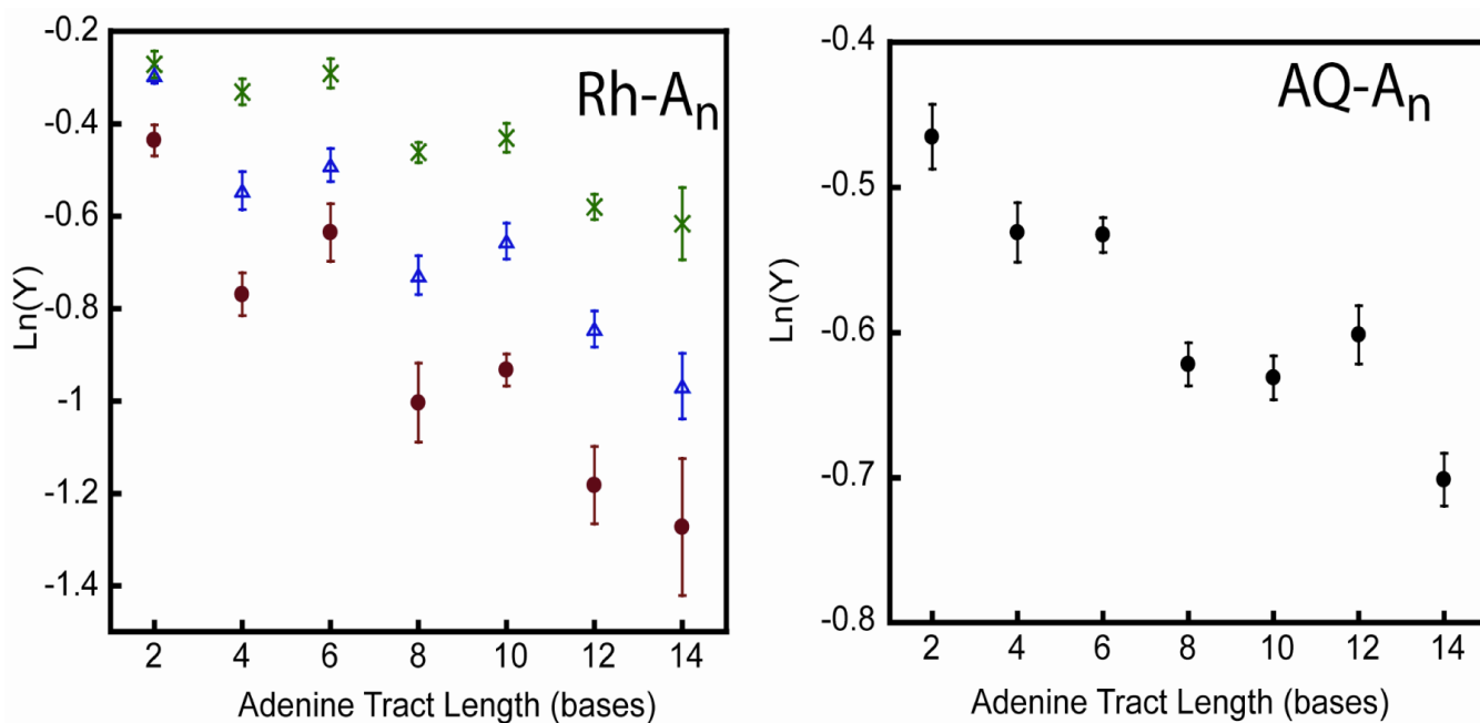
Figure 3. CT yields ( Y ) as a function of bridge length for the Rh-A n series and AQ-A n series. Results at three temperatures are shown for the Rh-A n series: 20 °C (red circles), 30 °C (blue triangles), and 40 °C (green x's); AQ-A n experiments are at ambient temperature. Duplexes (10 μM) were irradiated at 365 nm in 20 mM sodium phosphate, 50 mM NaCl, pH 7.0 as described in the text. The bridge length is defined as the number of adenines between the photooxidant and the trap. The experiments were repeated at least three times, the results averaged, and the error is expressed as 90% confidence intervals of the mean.
