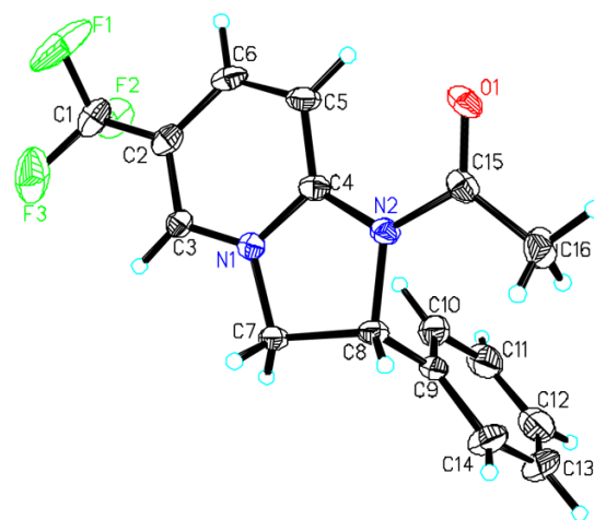
X-ray structure of 5a
